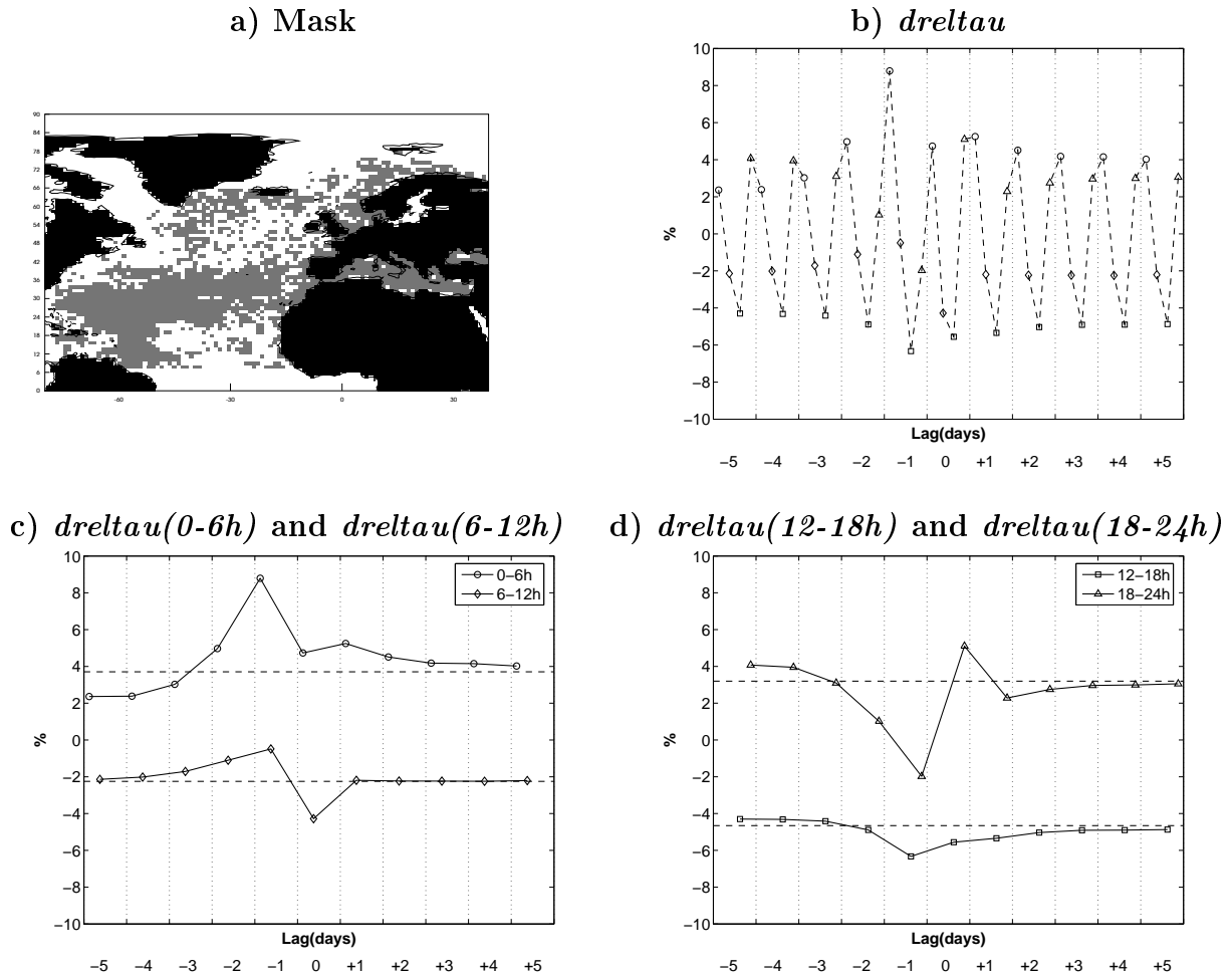
FIG. 5.12 – a) Mask : In grey, area where the composites of dreltau , selecting the days for which dtemp > std(dtemp) , reach the 95% significance level at day -1, according to a bootstrap test. dreltau and dtemp are defined in the text. b) Spatial average over the mask in a) of these composites of dreltau . c) Time series of the 0-6h and 6-12h values from a) with their seasonal mean (dotted line) d) Time series of the 12-18h and 18-24h values of from a) with their seasonal mean (dotted line). Day 0 is a day for which dtemp is higher than its standard deviation.
