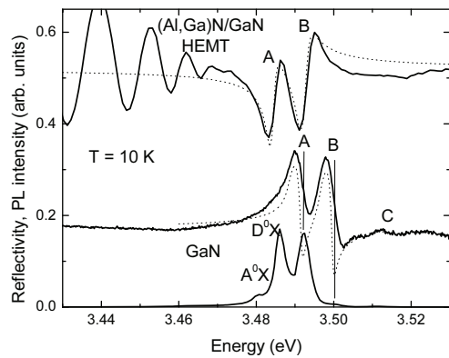
Figure 1 Low temperature PL and reflectivity spectra of a GaN sample and reflectivity spectrum of an HEMT structure. Dotted lines are calculated reflectivity spectra.
