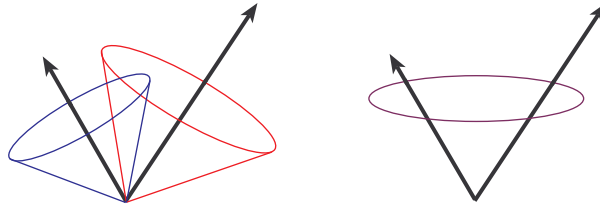
Figure 1.35: Jet reconstruction algorithms using different R_{cone} values. (left) A jet algorithm with a smaller R_{cone} can discriminate between 2 jets that are found close in \Delta R while (right) only one jet is reconstructed in the case of a higher R_{cone} .
