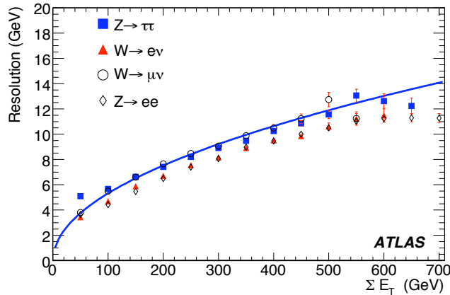
Figure 1.34: Resolution of the two \cancel{E}_T components with refined calibration as a function of the total transverse energy, \Sigma E_T [19].
