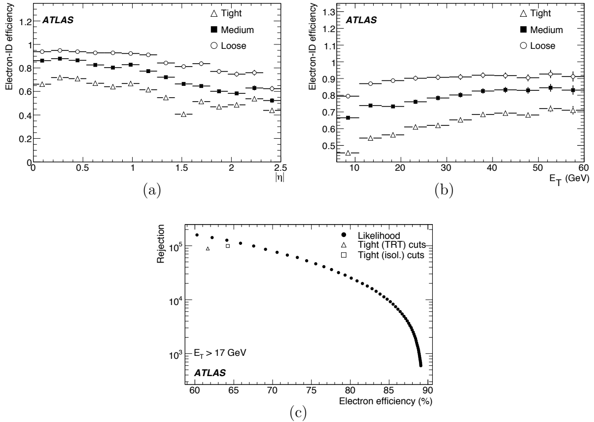
Figure 1.25: Electron identification efficiency as a function of |\eta| (a) and E_T (b) for electrons with E_T > 5 GeV from H \rightarrow eeee decays. Jet rejection versus isolated electron efficiency obtained with a likelihood method compared to the results from the two sets of tight cuts. Only electrons with E_T > 17 GeV are selected in this case (c). [19].
