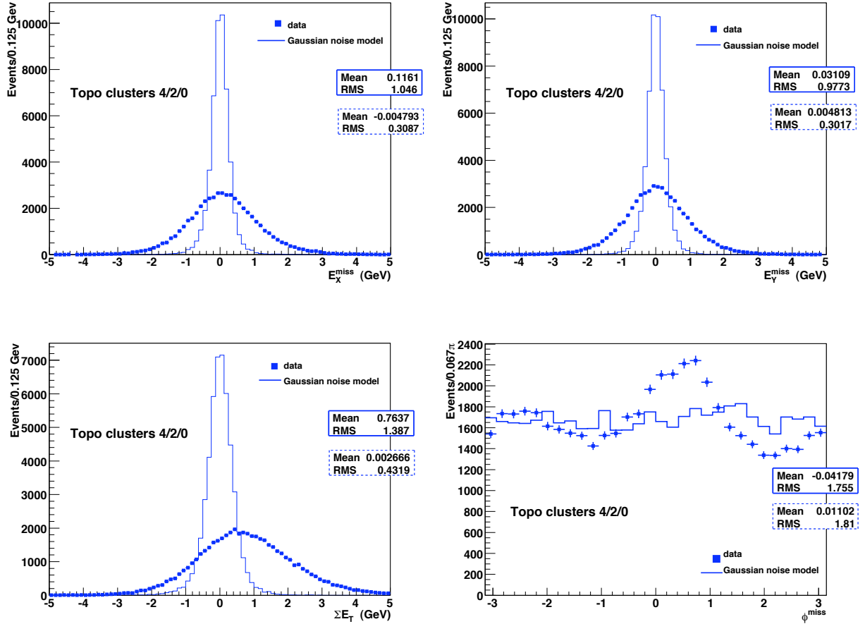
Figure 2.18: E_X^{miss} , E_Y^{miss} , \Sigma E_T and \phi^{miss} distributions computed with topocluster cells for random events of the reference run (91639). Blue dots represent the data, whereas the solid line is the toy Monte-Carlo.
