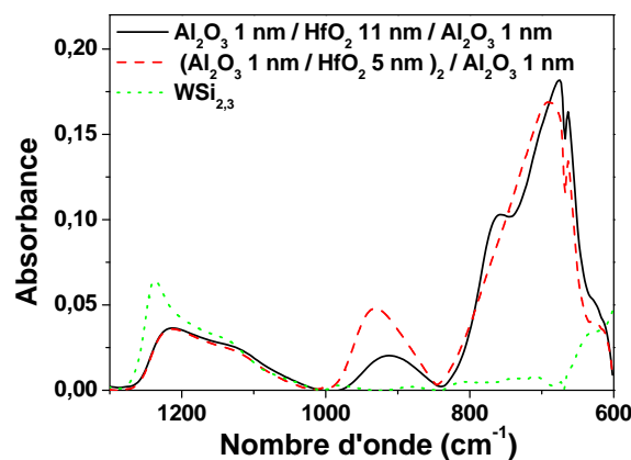
FIG. 5.6 – Spectres ATR en absorption (a) de la structure sandwich \text{Al}_2\text{O}_3 1 nm / \text{HfO}_2 11 nm / \text{Al}_2\text{O}_3 1 nm et nanolaminate \text{Al}_2\text{O}_3 1 nm / \text{HfO}_2 5 nm / \text{Al}_2\text{O}_3 1 nm / \text{HfO}_2 5 nm / \text{Al}_2\text{O}_3 1 nm.
