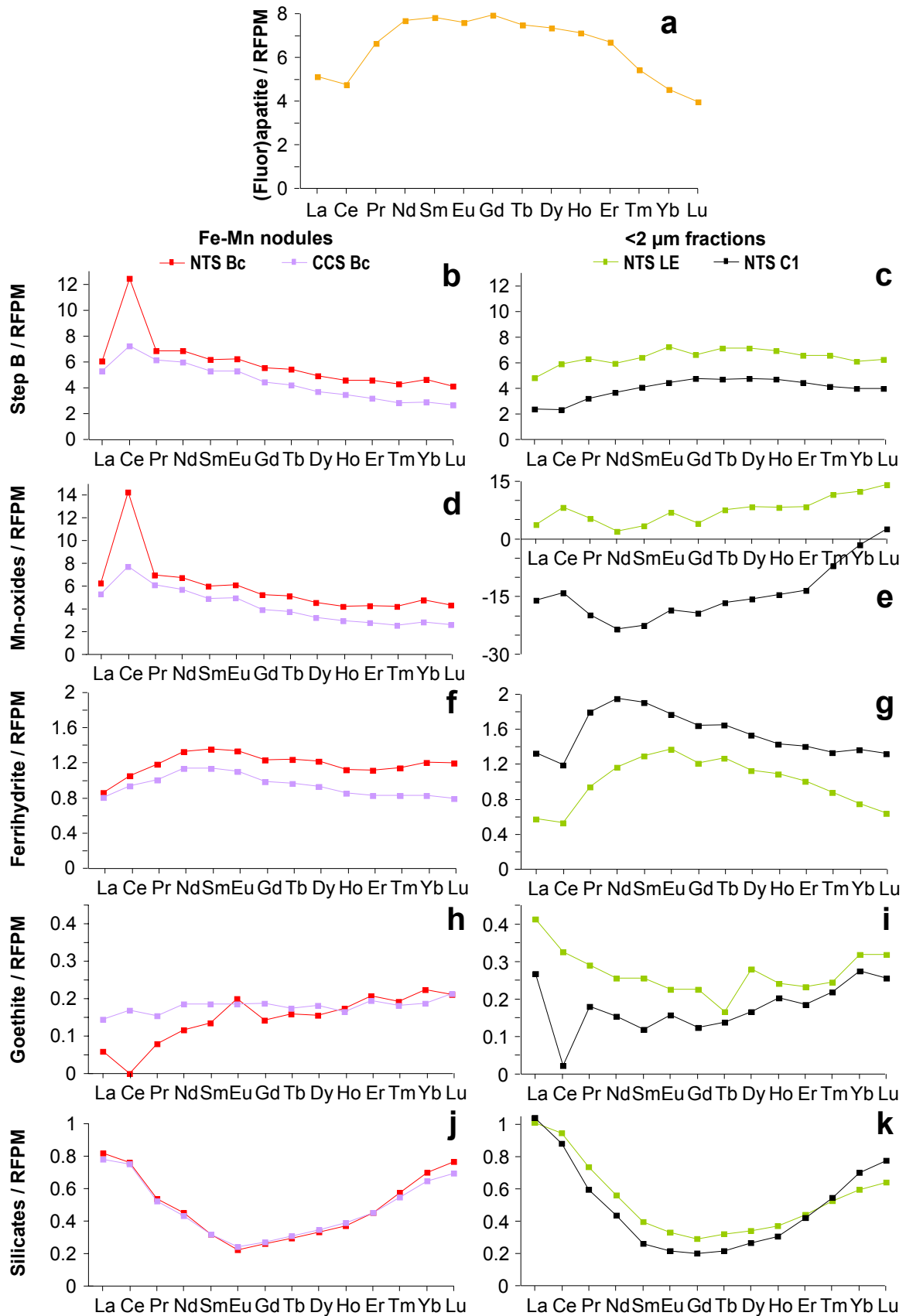
Figure 7. REE concentrations in reconstructed (fluor)apatite, Mn-oxides, ferrihydrite, goethite, and silicates of the Fe-Mn nodules and of the <2 μm fractions normalized to the REE concentrations in the residues of former parent materials (RFPMs) of their respective soil horizons, as calculated by Laveuf et al. (submitted, cf. Chapitre 5.1.).
