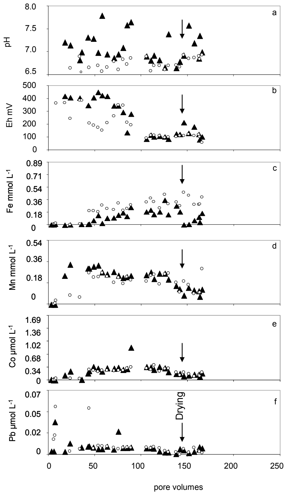
Figure 7: pH, Eh, Fe, Mn, Co and Pb concentrations as a function of the pore volume of the inflow and outflow for the quartz column undergoing 14-day cycles. Dark triangles represent the outflow, while open circles are for the inflow.
