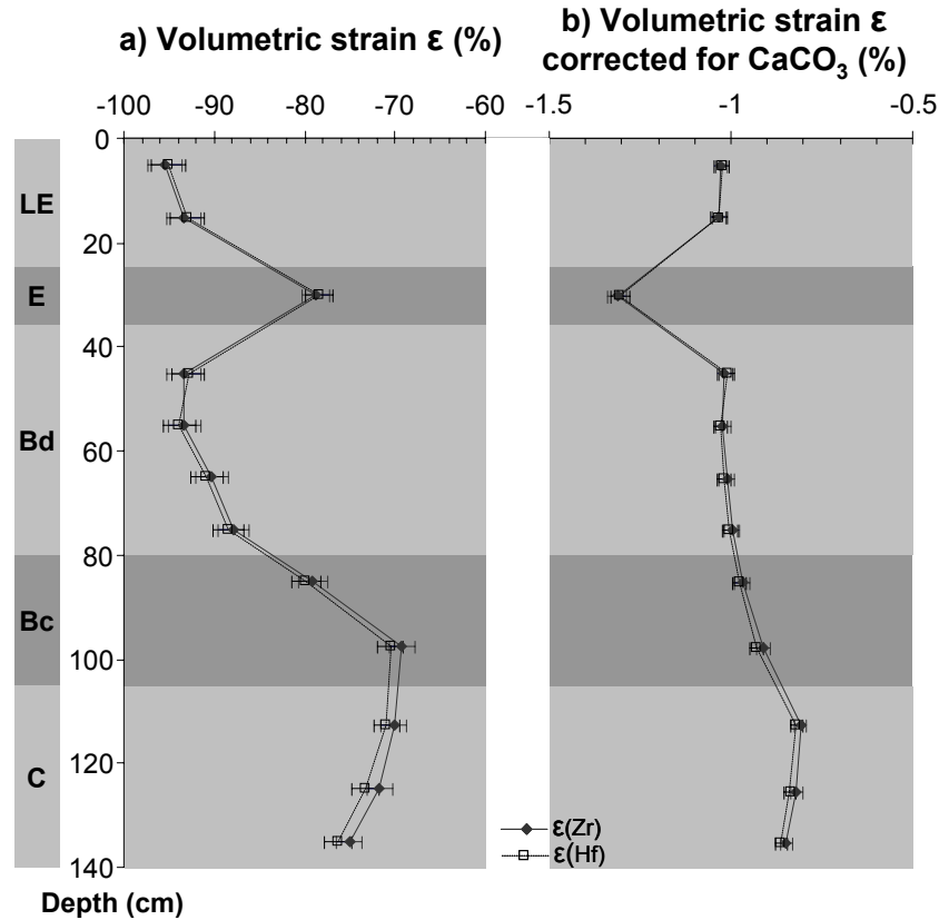
Fig. 5. (a) Calculated volumetric strain \varepsilon (in %) along the studied solum using Zr and Hf as immobile elements. (b) Calculated volumetric strain normalized to the \text{CaCO}_3 contents of the corresponding former parent material reconstructed for each soil horizon.
