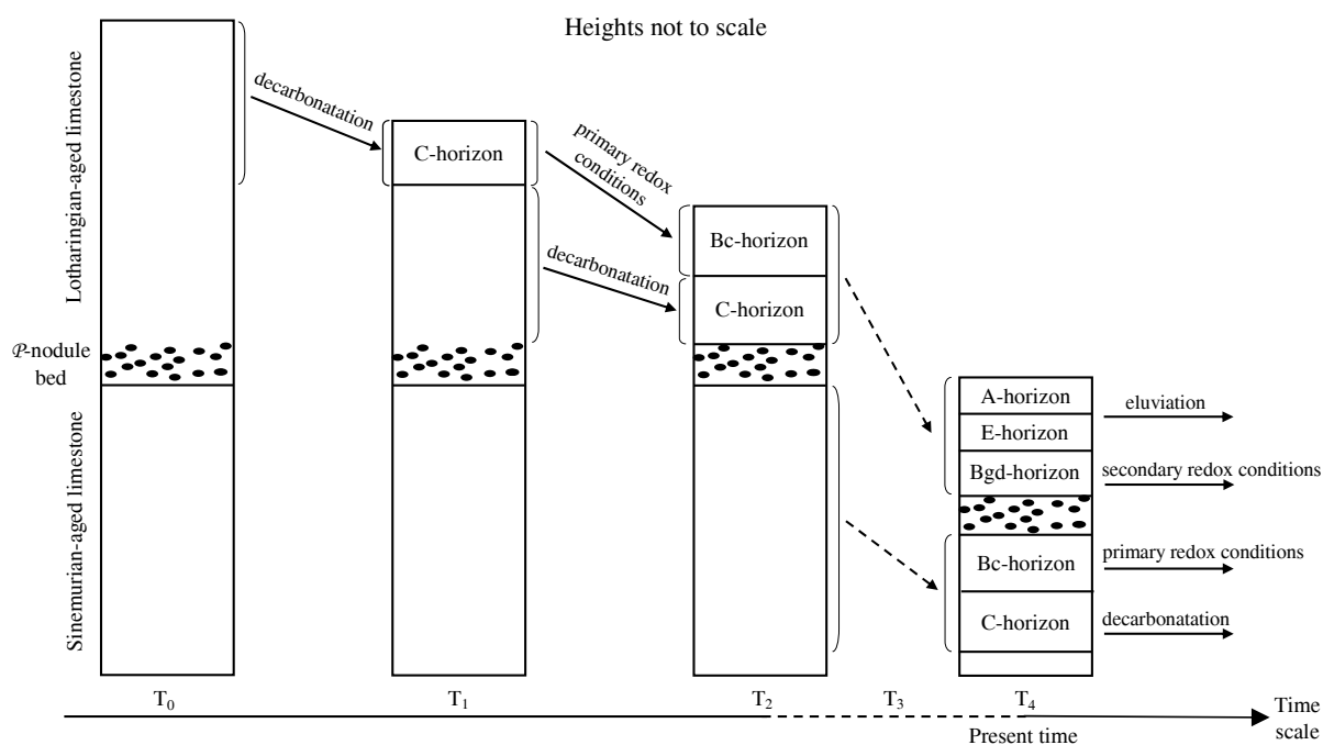
Fig. 1. Pedogenesis of the studied solum based on the vertical transformation fronts of the successive pedogenetic processes. Processes identified by Baize and Chrétien (1994) and Laveuf et al. (2009, cf. Chapitre 3.1.).
