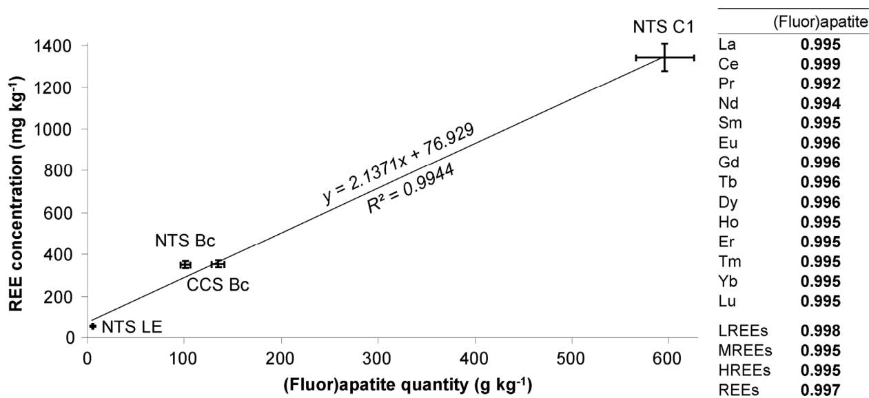
Figure 6. Concentrations of REEs in the non-magnetic >50 \mu\text{m} fractions as a function of their (fluor)apatite contents and Pearson's correlation coefficients of individual and groups of REEs with (fluor)apatite. Significant correlation coefficients at the threshold of \alpha=0.05 are reported in bold.
