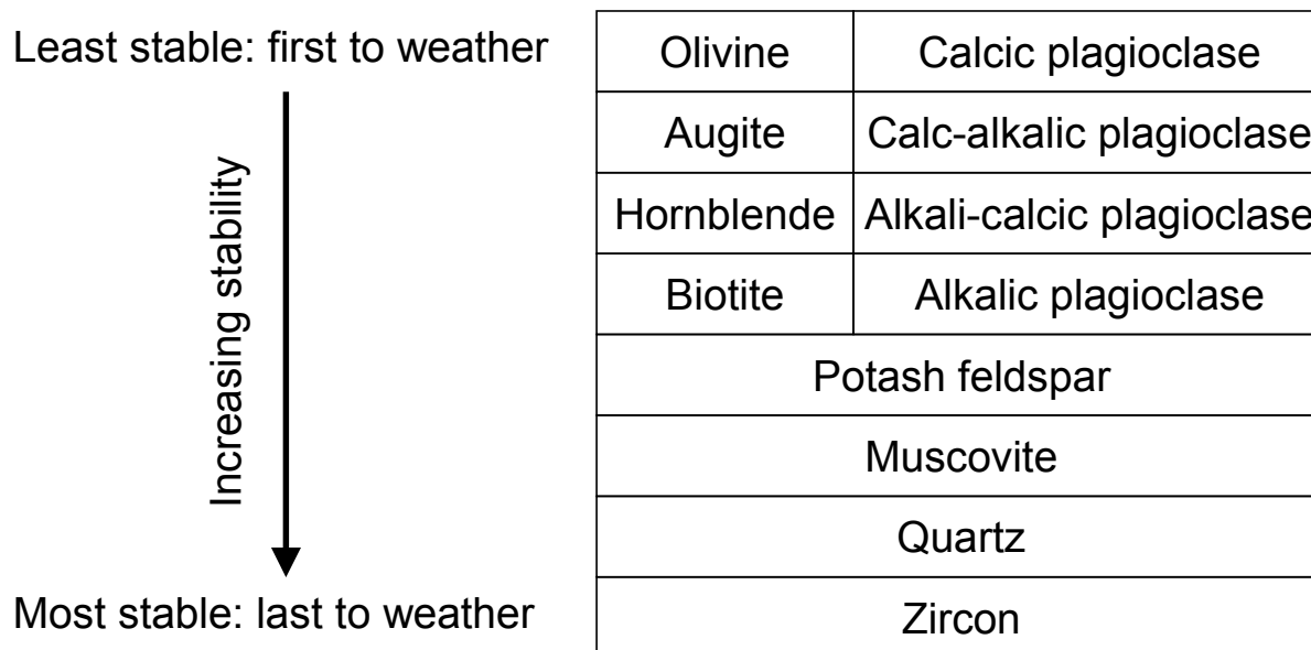
Fig. 1 Weathering sequence of primary minerals (after Goldich, 1938).
