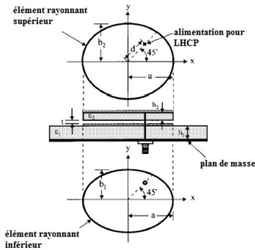
Figure 3.12: Antennes elliptiques
