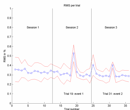
Figure 3: RMS on position results
