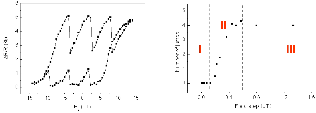
Figure 18 : Left: Voltage variation in the MR for an applied field of -15/+15 \mu\text{T} scanned on 100 points. The corresponding field step is 0.6 \mu\text{T} . Right: Number of jumps as a function of the field step applied to the sample for the Nb-B device. The field has been scanned between -10 and +10 \mu\text{T} at different rate.
