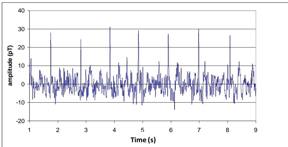
Figure 24 : Raw MCG signal recorded on a Nb-mixed sensor with a thermal noise of 100 fT/ \sqrt{\text{Hz}} .
