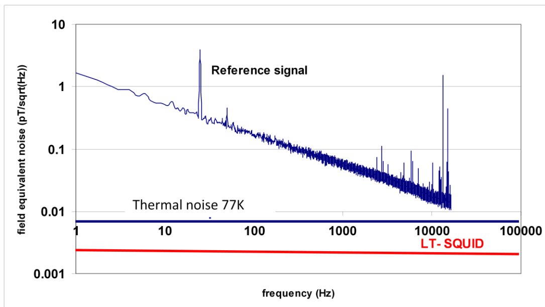
Figure 17: Field equivalent noise recorded in the MSR with a YBCO sensor at 77 K, and with a reference signal of 5 pT at 30 Hz produced by a small dipolar coil. The thermal noise of the sensor is indicated by the plain blue line. Low-Tc Squids detectivity level is indicated by the red plain line.
