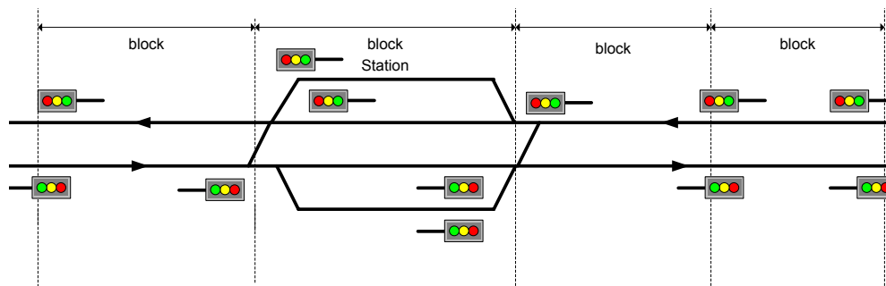
Figure 3.6: Representation of the block system.
