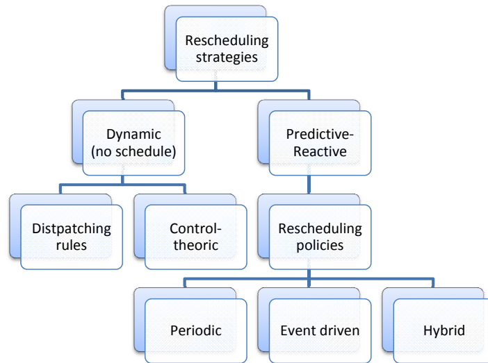
Figure 3.4: Rescheduling Framework: Strategies (Vieira et al., 2003)
