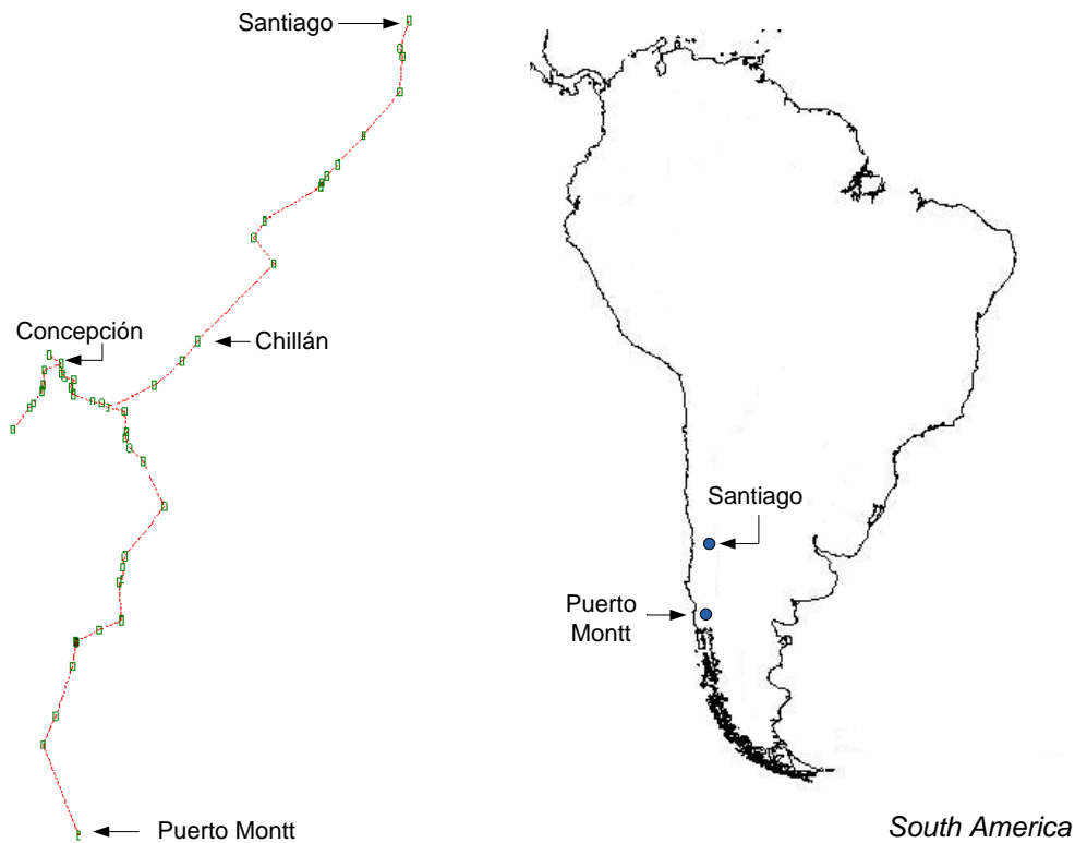
Figure 4.7: Network 2. Left: Stations and sections of the network. Right: Location of the network in Chile.
