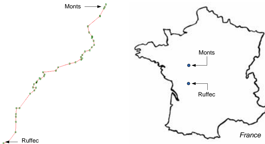
Figure 4.4: Network 1. Left: Stations and sections of the line. Right: Location of the line in France.
