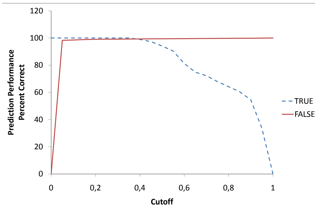
Figure 5.3: Prediction performance of the regression model.
