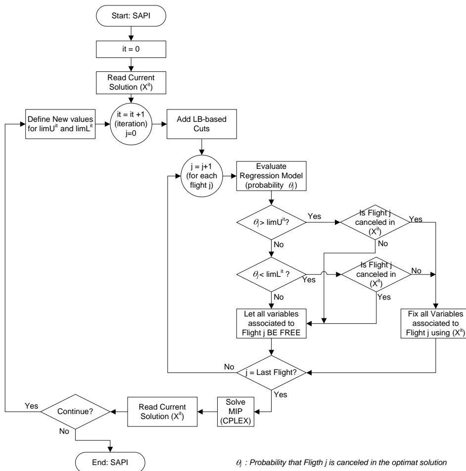
Figure 8.3: Flow diagram of function SAPI (Statistical Analysis of Propagation of Incidents).
