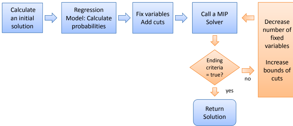
Figure 5.2: Sequential steps of Iterative SAPI method
