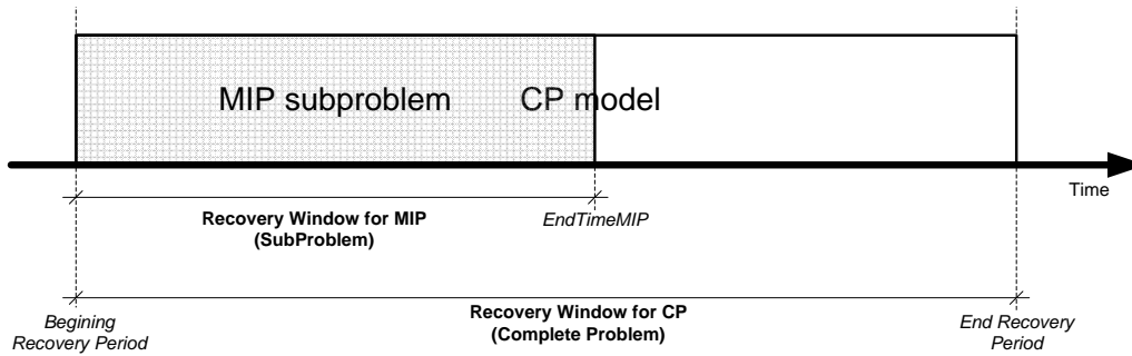
Figure 6.2: Relation between the complete CP model and the MIP subproblem.
