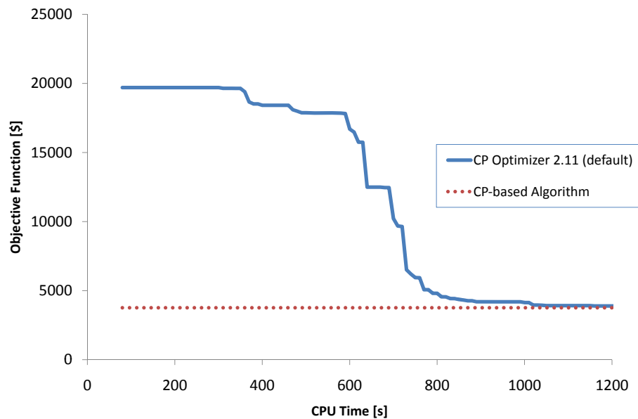
Figure 6.5: Comparative analysis for instance france-1-a-10 . CP Optimizer 2.11 versus Algorithm 4
