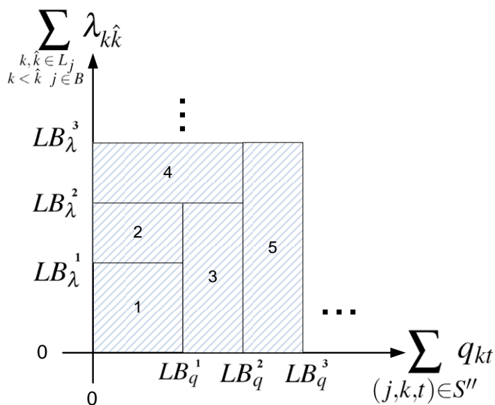
Figure 4.3: Search space of Iterative MIP-based local search. The numbers in the areas represent the feasible search space at each iteration.
