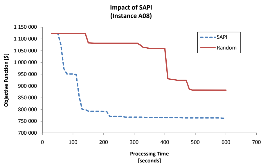
Figure 8.6: Impact of SAPI. This graph shows two different version of the algorithm: a) SAPI with a logistic regression b) random selection of flights
