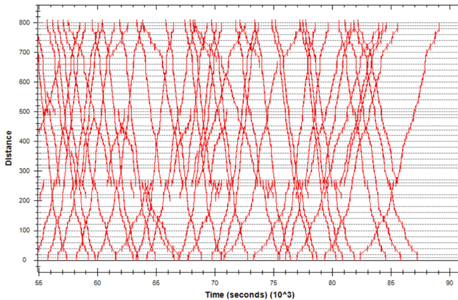
Figure 4.5: Traffic diagram for Network 1 (France). Every line represents a train, x-axis corresponds to the time in seconds, and y-axis represents a relative distance (without real units).
