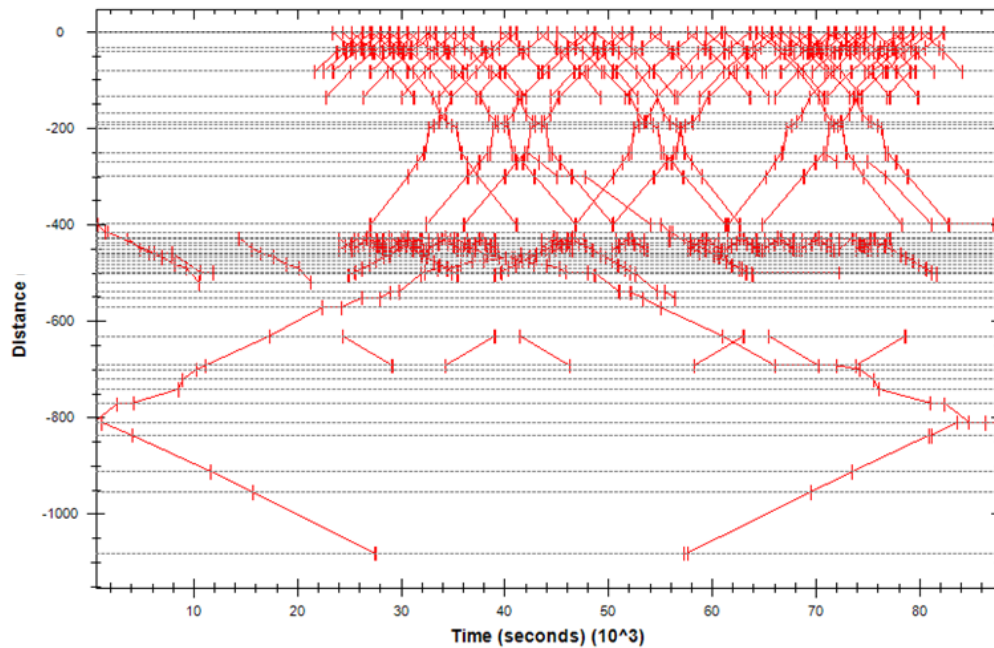
Figure 4.8: Traffic diagram for Network 2 (Chile). Every line represents a train, x-axis corresponds to the time in seconds, and y-axis represents a relative distance (without real units).
