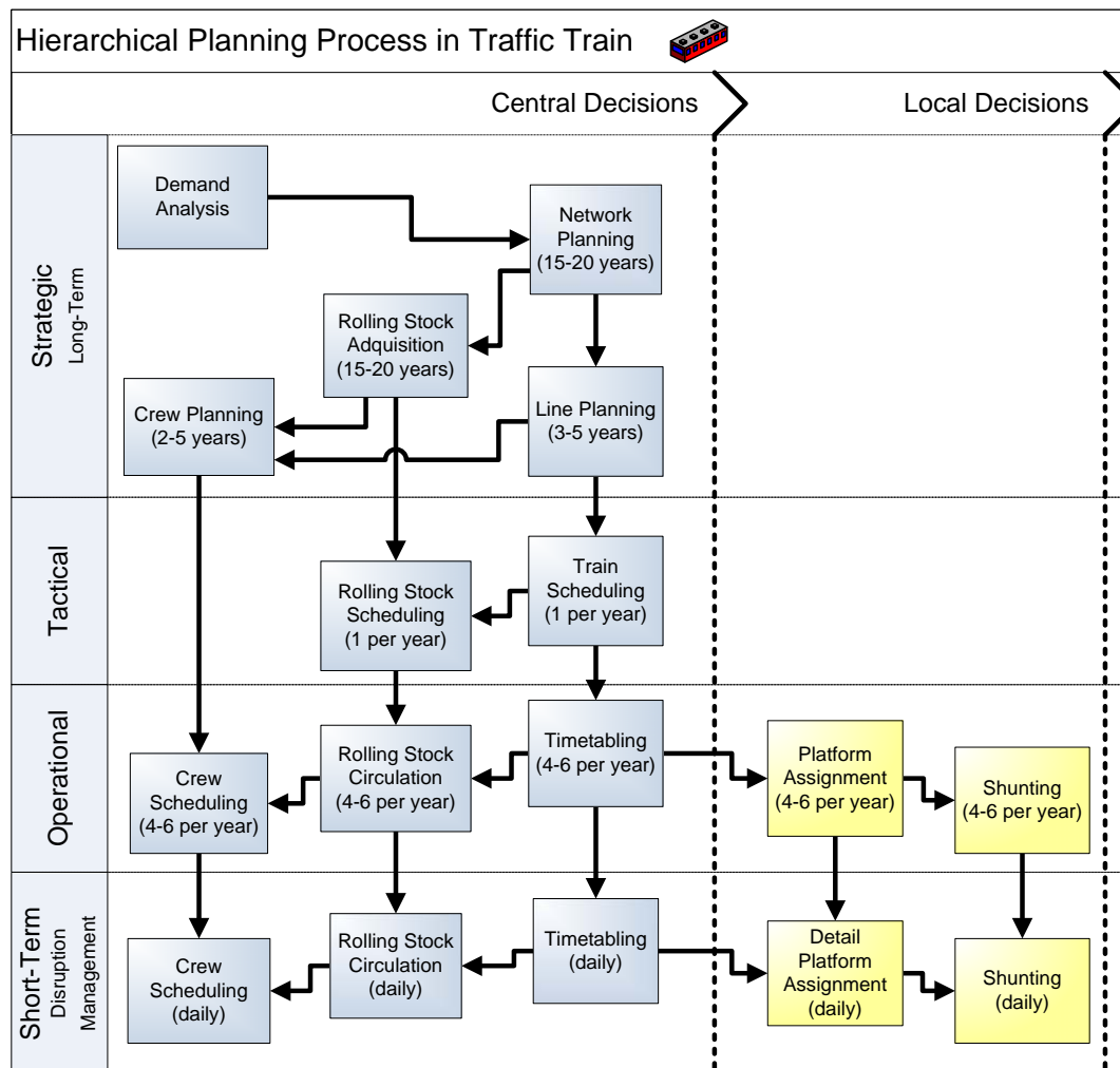
Figure 2.1: Two-dimensional classification of rail transportation problems
