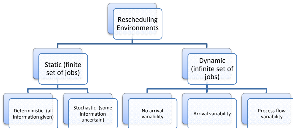
Figure 3.3: Rescheduling Framework: Environments (Vieira et al., 2003)
