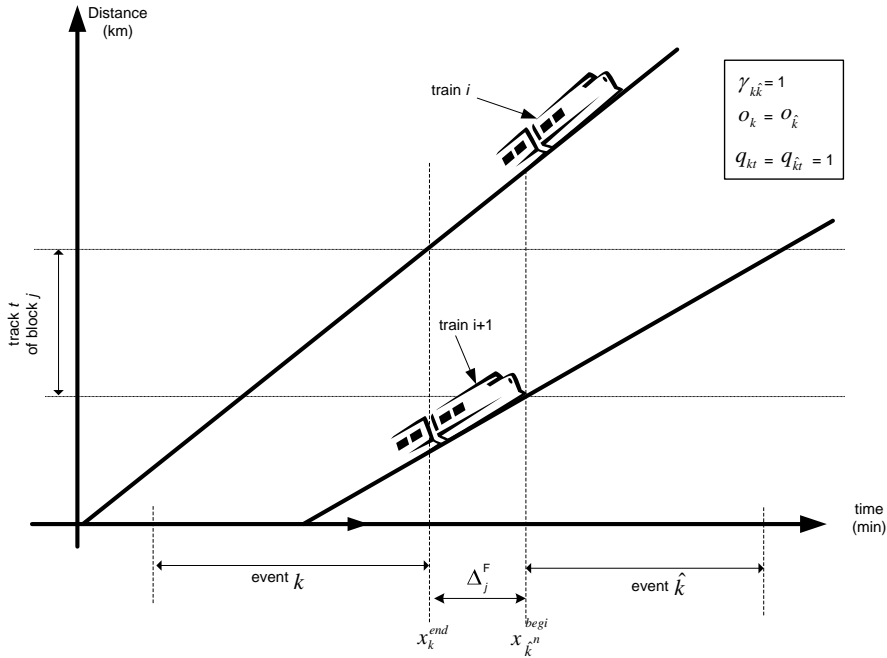
Figure 4.2: Time-distance diagram: An example for variables and constraints in the MIP model
