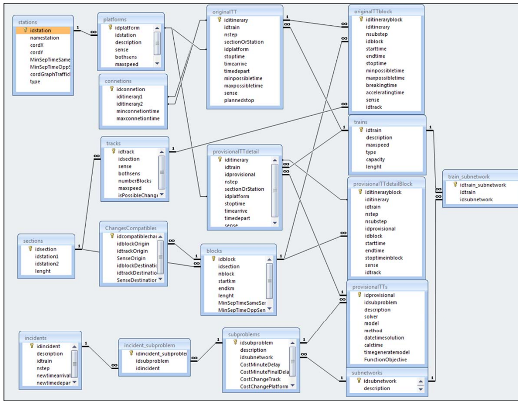
Figure 10.1: Database design.
