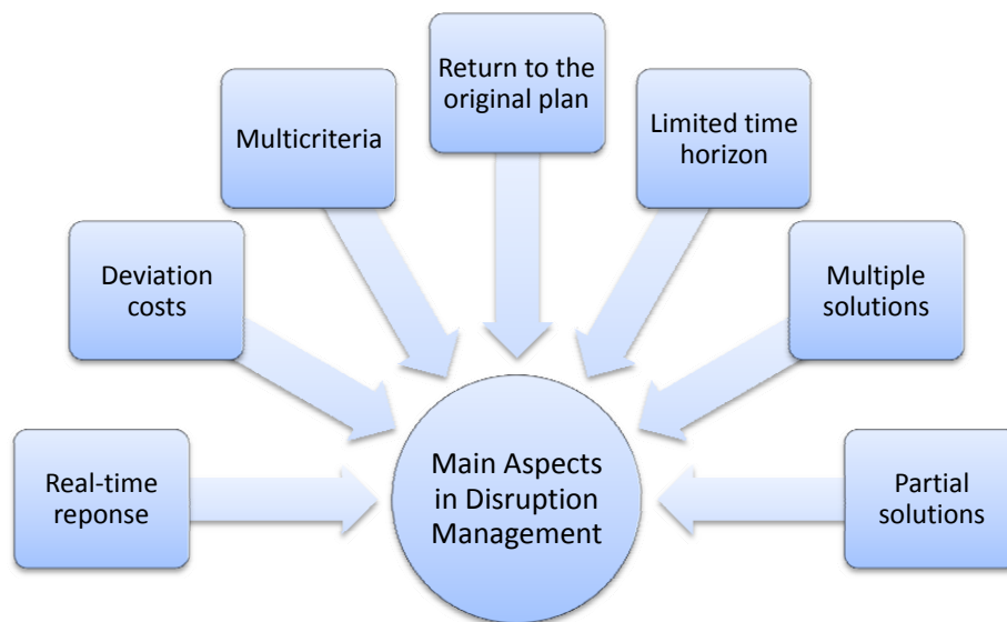
Figure 3.2: Aspects in Disruption Management
