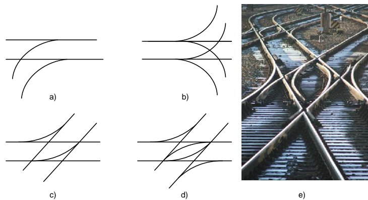
Figure 3.7: Different type of junctions: a) simple branching, b) triple branching, c) simple crossing junction, d) double crossing junction, e) real double crossing junction ( Flickr.com, 2006 )
