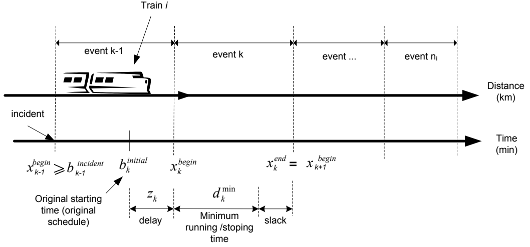
Figure 4.1: Illustration of time variables, parameters and constraints
