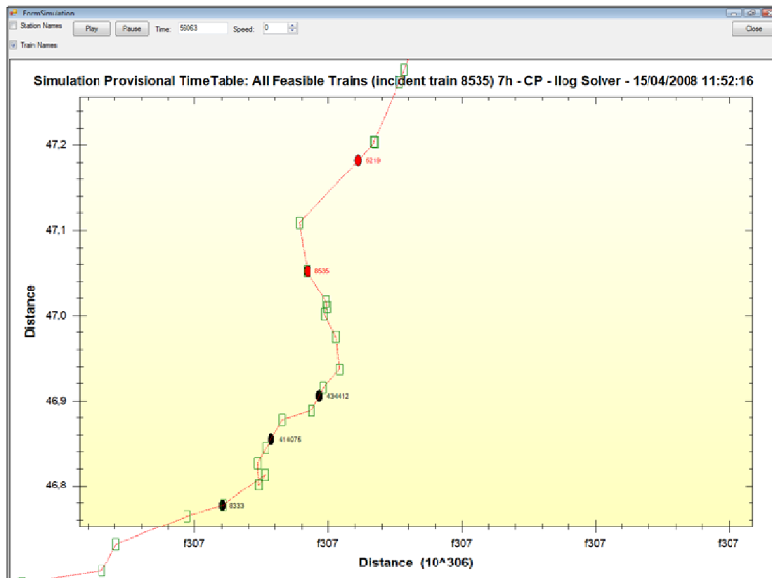
Figure 10.8: Simulation: One of the visualization tools is Simulation. In this screen, users can simulate both: original and provisional timetables. The user is able to modify the speed, the scale, and other parameters of the simulation. One train can have three colors: black, red and green. The first one is used to represent a train in movement that is on time. Red trains are delayed trains moving. Finally, green trains correspond to trains stopped in a station.
