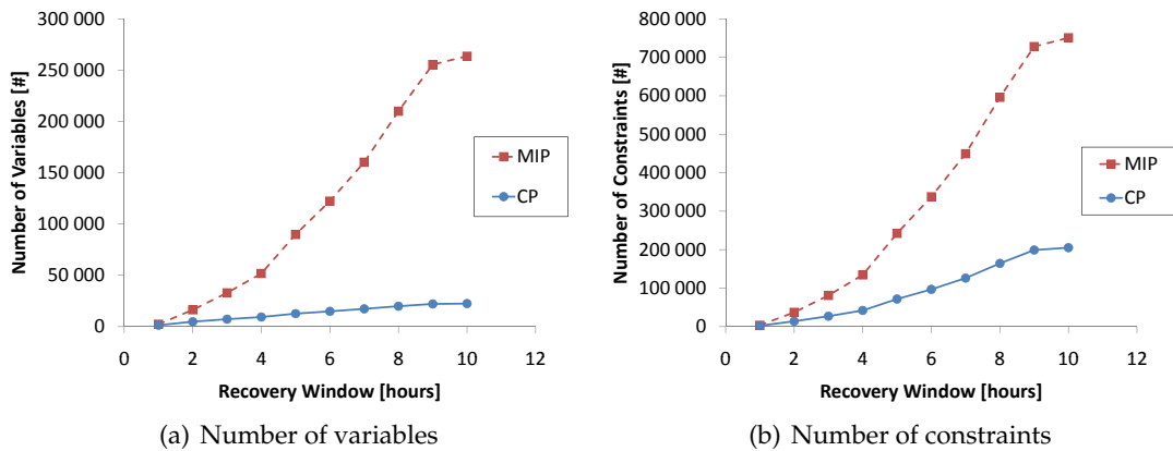
Figure 6.1: Differences of the size of the models size: MIP vs. CP
