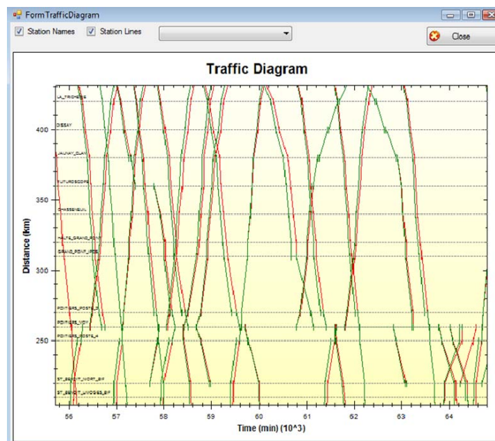
Figure 10.7: Visualization Tool: This screen shows a typical solution of the problem. Green lines are the original schedule of trains and red lines are the provisional timetable. The horizontal distance between the red and green line for one train represents its delay.
