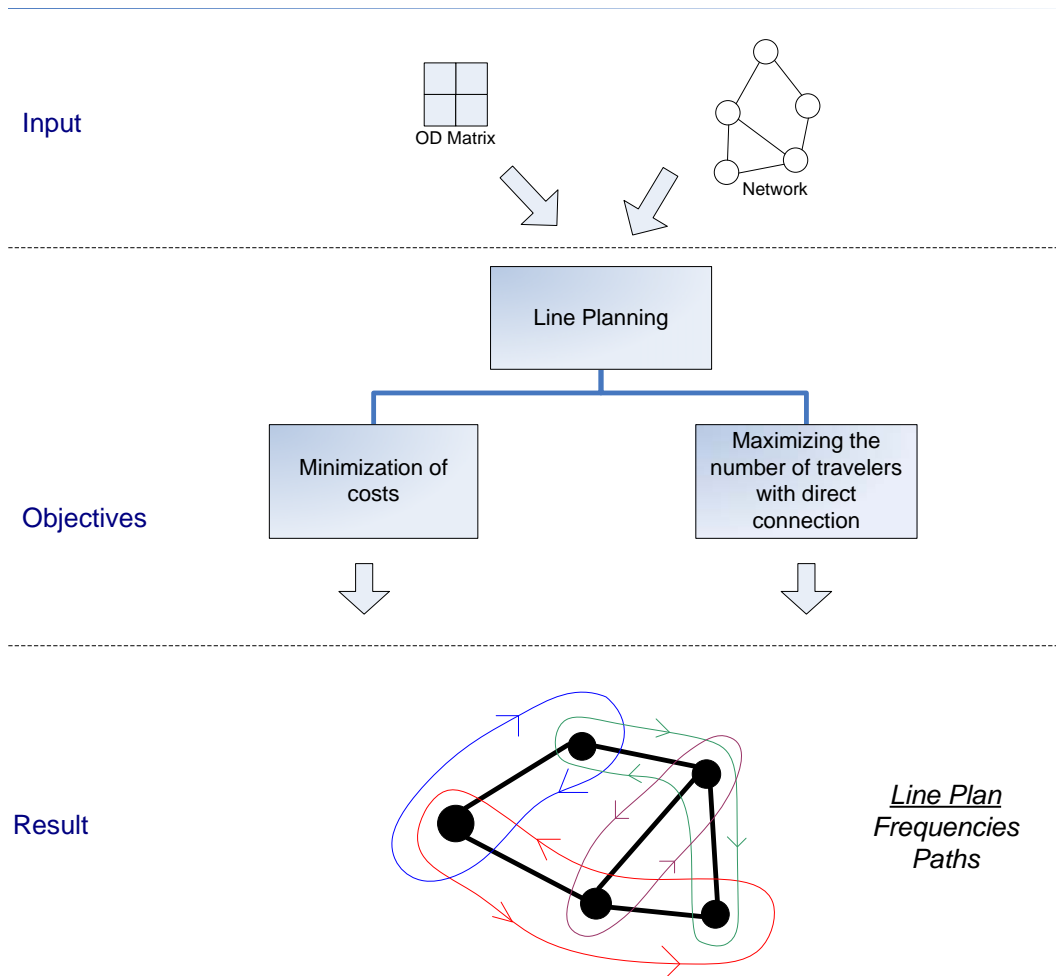
Figure 2.2: The Line Planning Problem.
