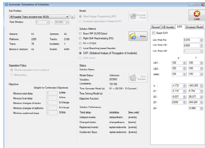
Figure 10.6: Automatic generation of timetable: This window permits the user selects a sub-problem and to choose a solution method. The system reads the information from the database and generates an appropriate mathematical model depending on the solution method selected
