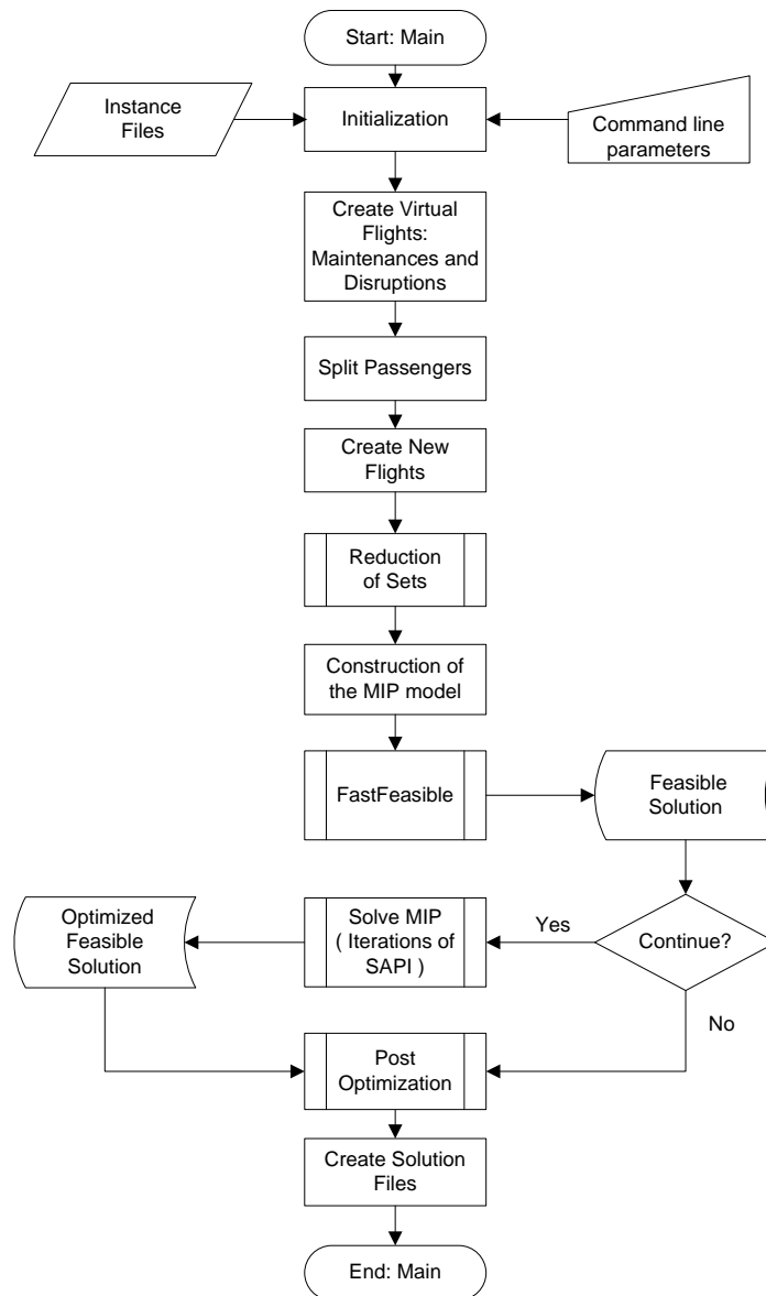
Figure 8.2: Flow diagram of the solution method.
