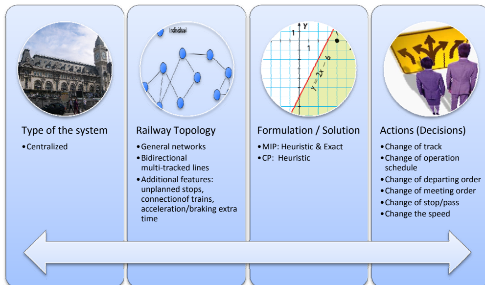
Figure 3.8: Scope of this Thesis: type, topology, formulation & solution, and actions
