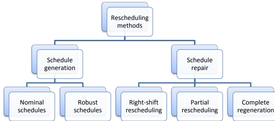
Figure 3.5: Rescheduling Framework: Methods (Vieira et al., 2003)
