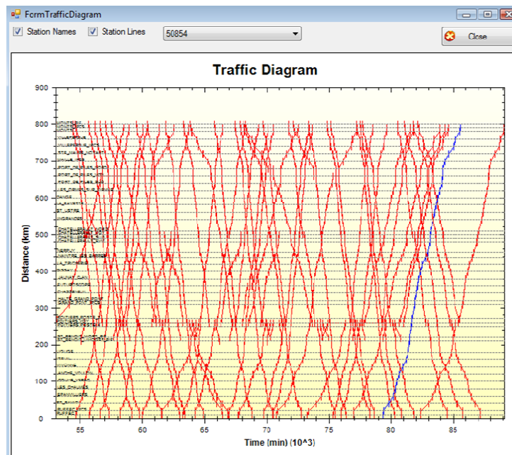
Figure 10.5: Traffic Diagram: This is one of the most used graphics in train transportation. It is a two dimensional chart with the time in the x-axes and the distance in y-axes. The red lines represent trains, and also there are horizontal lines representing the stations
