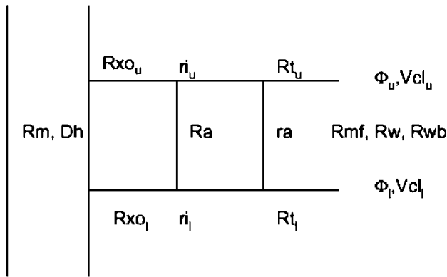
Fig. 3—A bed is described by a set of parameters (i.e., physical and petrophysical properties). In addition to standard resistivity description, the user can choose more complex models in which resistivity and petrophysical properties are linked through a saturation equation (refer to the Nomenclature for property definition— u stands for upper, l for lower).
