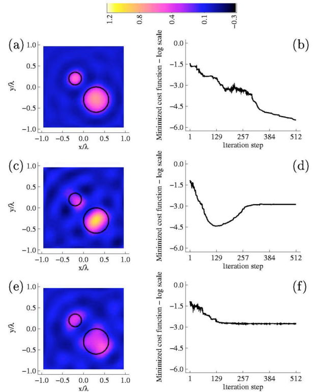
Fig. 3. (Color online) Reconstructed contrast distribution using a conjugate-gradient method, for the HOMO CYL16 object. The updating direction d_n involves a gradient derived from a solution of an adjoint problem. (a) Both the internal field and the adjoint field are computed accurately (FULL–FULL case); (c) same as in (a) but the evaluation of the adjoint field assumes the Born approximation (FULL–BORN case); (e) the Born approximation is assumed for both the internal field and for the adjoint field (BORN–BORN case). Curves (b), (d), and (f) represent the evolution in logarithmic scale of the minimized cost functional with respect to the iteration steps for the reconstructions plotted in (a), (c), and (e), respectively.
