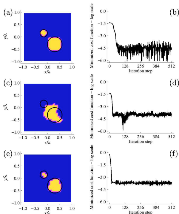
Fig. 8. (Color online) Same as in Fig. 6, but the inversion is performed using the level-set scheme described in Subsection 4.C.
