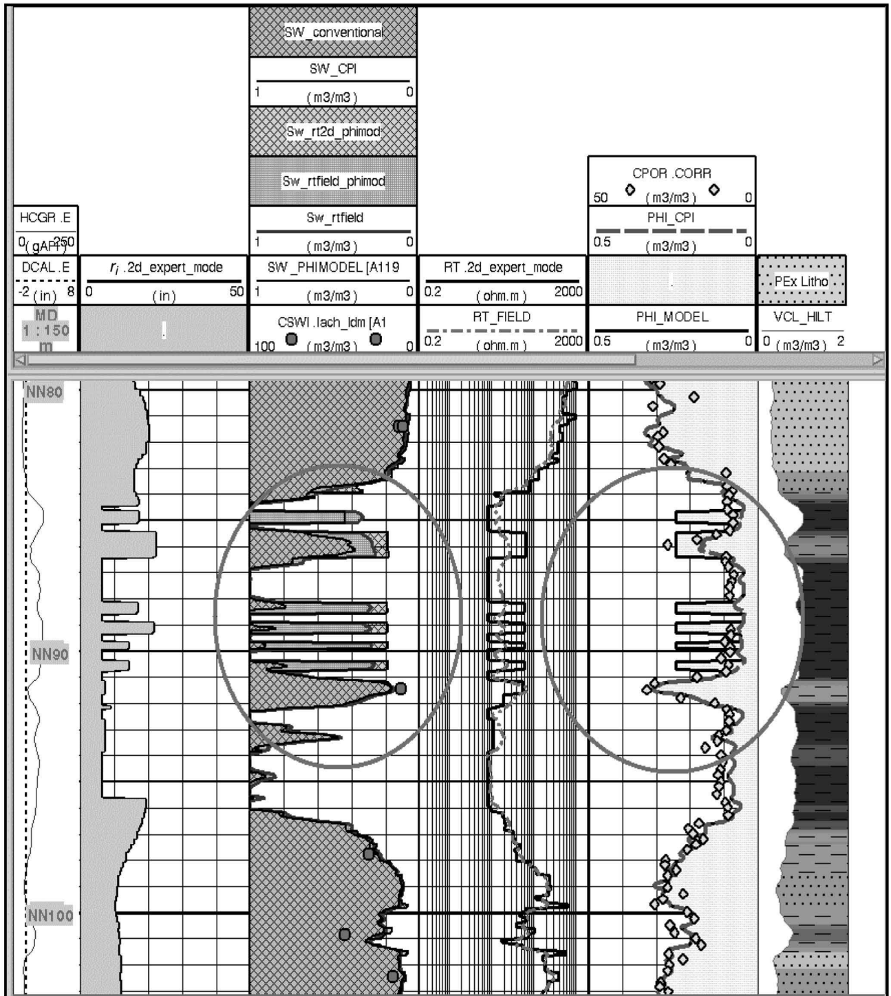
Fig. 11—Well 2: comparison of water-saturation profiles.
