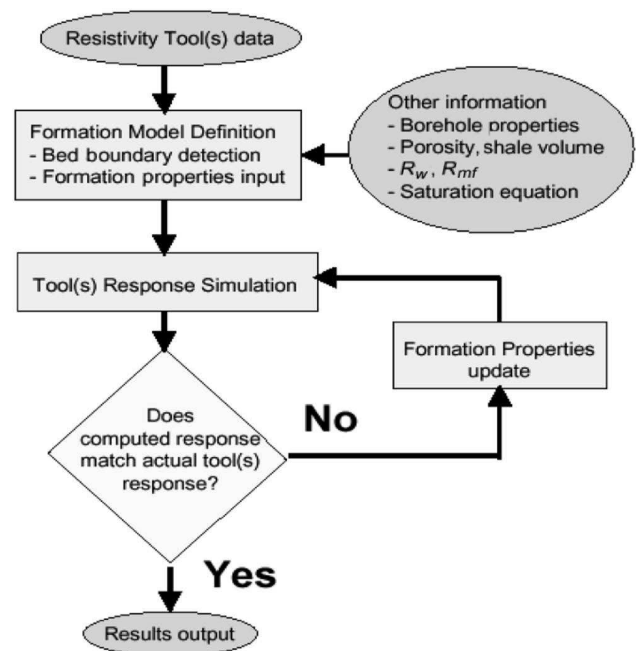
Fig. 2—Measurement-processing flow chart.
