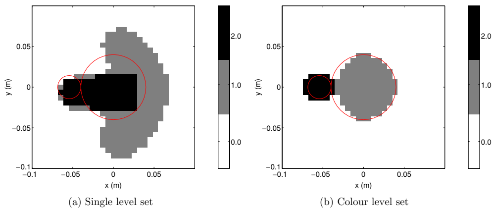
Figure 18. Resulting images for the FoamMetExt case.
