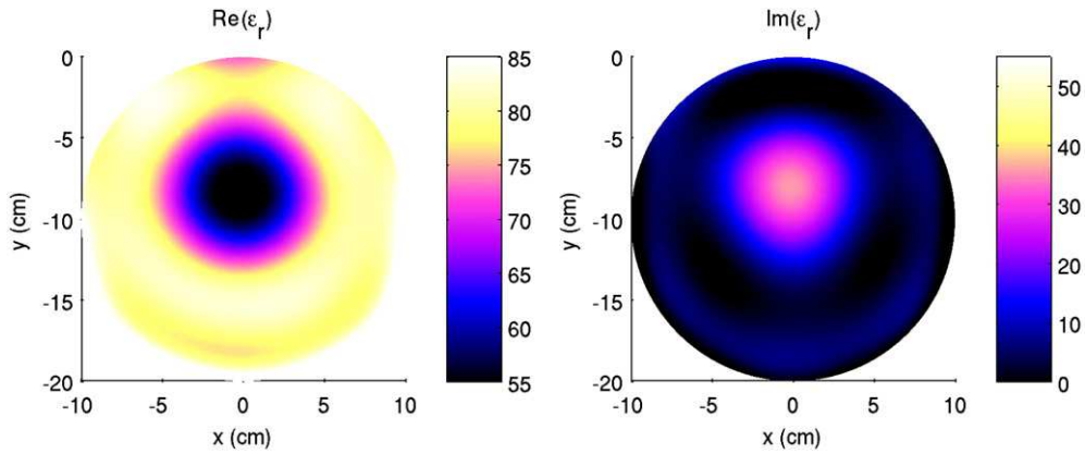
Figure 10. Real part (left) and imaginary part (right) of the permittivity map reconstructed after 100 iterations from a measured scattered field. The permittivity profile has been projected onto the Zernike polynomial basis with N_o = 6 . The initial guess is again the homogeneous background. A circular investigation area of 10 cm radius centered at (0, -10) cm is used.
