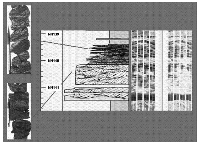
Fig. 6—Tidal-influenced channel.
