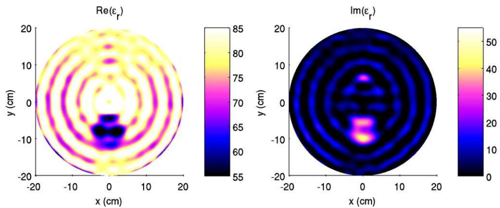
Figure 4. Real part (left) and imaginary part (right) of the permittivity map reconstructed after 100 iterations from a measured scattered field. The value of the permittivity in each discretization cell is taken as an unknown in the inversion scheme. A large centered investigation area of radius 20 cm is taken.
