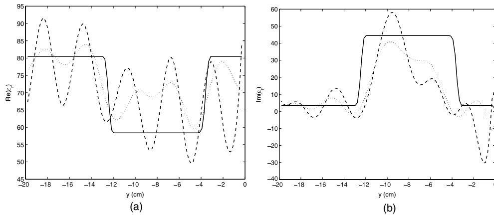
Figure 7. Real part (a) and imaginary part (b) of the permittivity profile reconstructed after 13 iterations ( \cdots ) and 100 iterations ( --- ). The profile has been obtained along the y -axis at x = 0 cm. The exact profile is also plotted ( — ). In the inversion process, the permittivity value in each discretization cell is taken as an unknown, the investigation area is the excentered disk of radius 10 cm.
