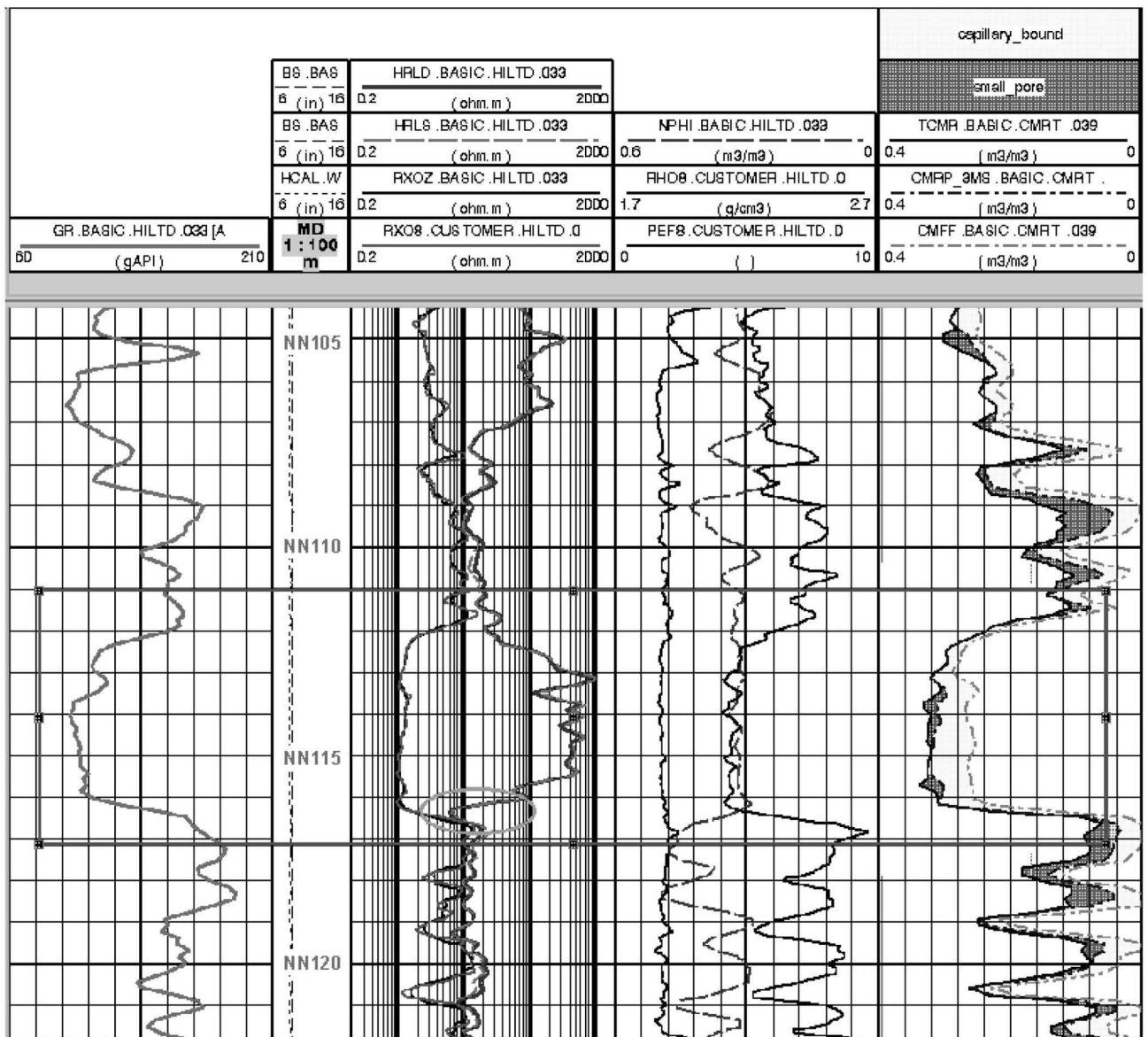
Fig. 7—Well 1: anomalous invasion or OWC?
