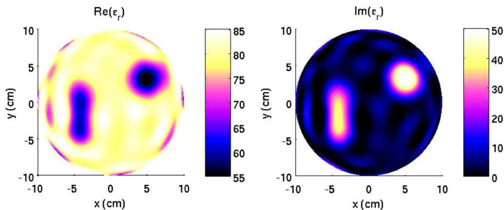
Figure 15. Real part (left) and imaginary part (right) of the permittivity map reconstructed after 100 iterations from a synthetic scattered field. White Gaussian noise with a signal-to-noise ratio of 10 dB has been added to the scattered field. The permittivity profile has been projected onto the Zernike polynomial basis with N_o = 12 . The initial guess is the homogeneous background. The investigation area is a disk of radius 10 cm, centered at (0, 0) cm.
