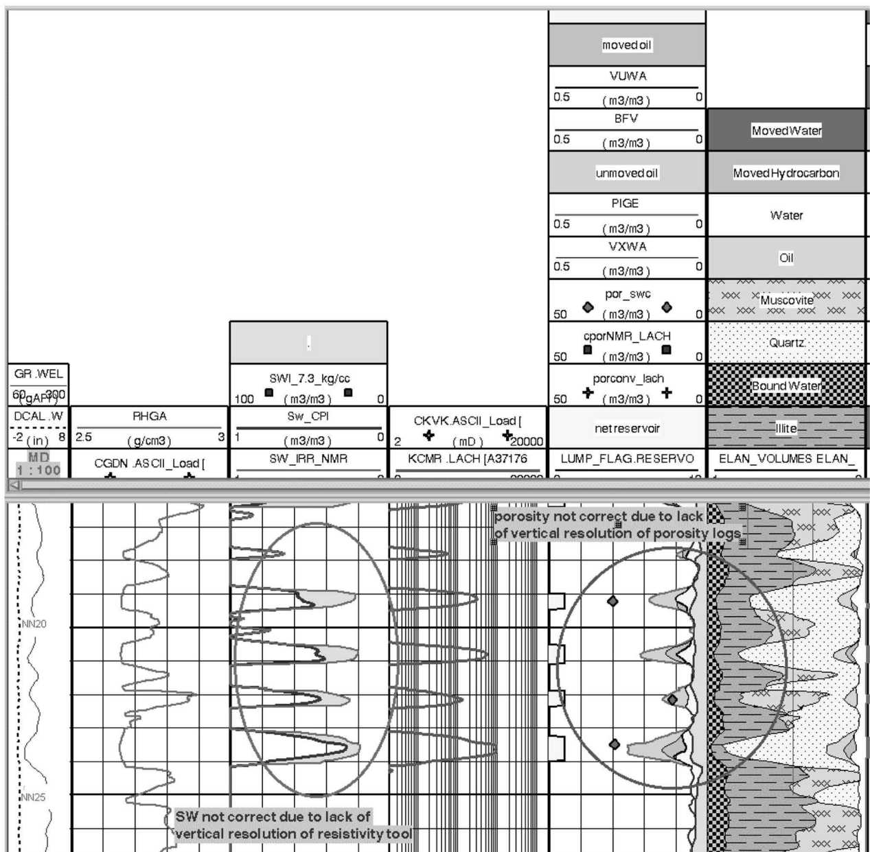
Fig. 9—Well 1—sequence of the thin beds: conventional interpretation. This example shows a conventional interpretation of wireline logs (computer-processed interpretation, or CPI). We can see that the estimated porosity is lower than core measurements (right oval) and that SW_{CPI} is higher than SW_{IRR} from NMR (left oval).
