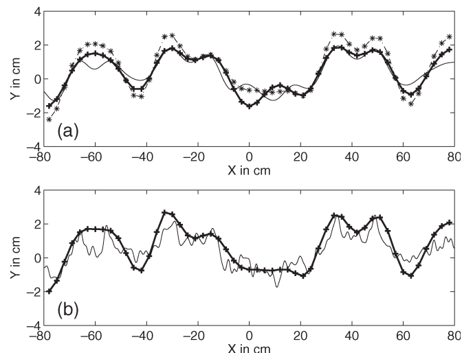
Fig. 2. Reconstructed surface profiles for the three test cases. (a) Gaussian surface profile corresponding to (line with stars) TC1 and (thick line with crosses) TC3. (b) Exponential surface profile corresponding to (thick line with crosses) TC2. The (thin lines) true profiles are also displayed.
