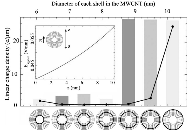
FIG. 3. Plot of the linear charge density associated with each shell of a MWCNT that is characterized by an inner and an outer diameter of 6.1 and 10.2 nm, respectively. The MWCNT is subjected to the same external electric field as in experimental conditions (see inset). The charges are provided by a reservoir representative of the tip that is situated just above the MWCNT at z = 10.2\text{ nm} . These results are obtained by applying the charge-dipole model of Ref. 18. The solid line indicates the results obtained when all shells are metallic. The other results (histograms) are obtained for MWCNTs for which only one shell out of three is metallic (no charge is carried by semiconducting shells). Three MWCNTs have been considered, with the outermost metallic shell, respectively, at the surface of the MWCNT (light gray) and one layer (medium gray) and two layers (dark gray) below the surface.
