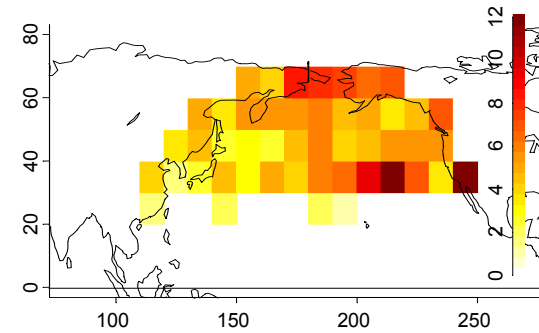
(f) Pression Dépressions ( \sigma ) [CNRM-CM3 XX1 - NCEP-NCAR] (hPa)
