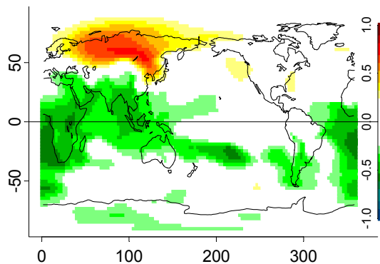
(h) Cor (Indice CP1-IA.CNRM-CM3, Ta2m&v10m)
