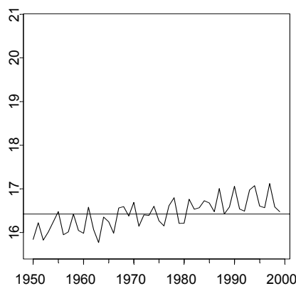
(a) Ta2m Globale CNRM-CM3 XX 1 (Moy. = 16.42^{\circ}\text{C} )
