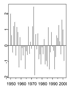
(i) CP2Tmax (20%)
