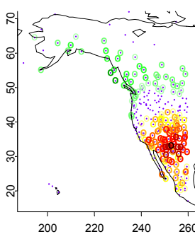
(j) Corrélations
