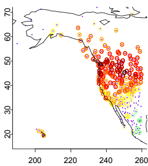
(j) Corrélations
