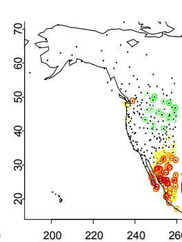
(k) Corrélations
