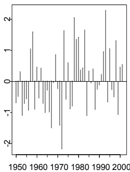
(j) CPR2FJP (12%)
