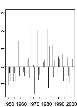
(j) CPR2FJP (12%)
