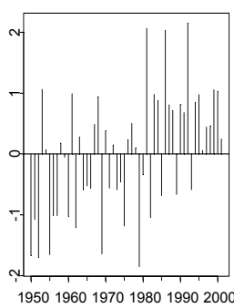
(i) CP2Tmax (20%)
