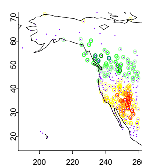
(h) Corrélations
