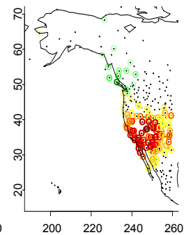
(k) Corrélations
