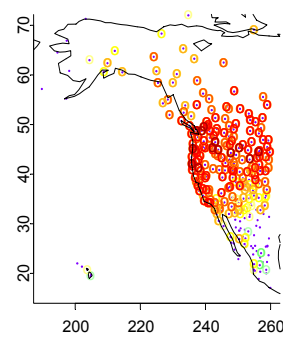
(h) Corrélations
