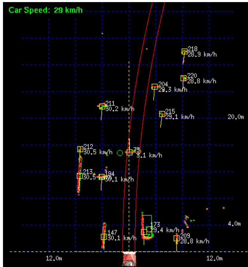
Figure 5.7: Interface of the perception module in action. The laser data is displayed as small colored points. Radar data is represented by small circles: left in green and right in yellow. Obstacles surrounding of the ego-vehicle are detected and represented by bounding-boxes of segments whose centers of gravity are highlighted by yellow squares. Note that all static and dynamic objects are all detected and their velocities plus movement directions relative to the car are computed and displayed next to each object along with objects ID.
