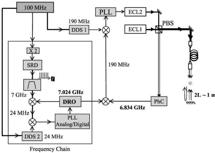
FIGURE 3 Scheme of the microwave synthesis and phase locked lasers. The 100 MHz quartz signal enters a frequency chain which generates the reference microwave frequency. Its microwave output is mixed with the lasers beatnote, and the IF is compared with a DDS signal. The error signal is used to phase lock the Raman lasers. ECL – extended cavity laser; DDS – direct digital synthesizer; PhC – photoconductor; SRD – step recovery diode; PBS – polarizing beam splitter; DRO – dielectric resonator oscillator
