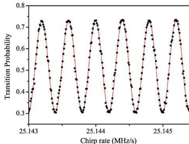
FIGURE 5 Atomic interferometer fringes obtained by scanning the Raman detuning chirp rate during the interferometer. The time between the Raman pulses is T = 50 \text{ ms} . The solid line is a sinusoidal fit of the experimental points displayed in black squares
