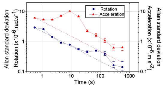
FIG. 5 (color online). Allan standard deviations of acceleration (triangles) and rotation (circles) measurements. Dashed lines correspond to the -1/2 slope expected for a white noise. The peak near 10 s averaging time on the acceleration signal is due to the residual oscillations of the isolation platform tilt.
