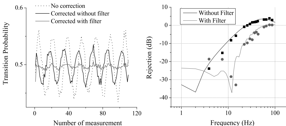
FIGURE 12 Left : modulation of the transition probability for an excitation frequency of 14 Hz, without correction, with correction, with and without a filter. Right : measured rejection efficiencies versus frequency, with and without a digital filter
