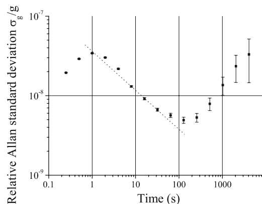
FIGURE 6 Allan standard deviation of the relative fluctuations of g . The time between the Raman pulses is T = 50 \text{ ms} . The dash line corresponds to a sensitivity of 3.5 \times 10^{-8} \text{ g Hz}^{-1/2}
