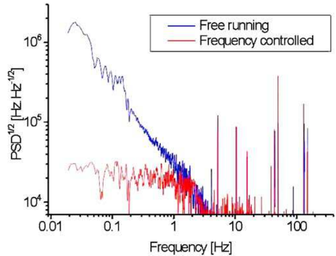
FIGURE 3 Power spectral density of the laser frequency noise in open- and closed-loop configurations. The data are derived from the error signal of the frequency-control system
