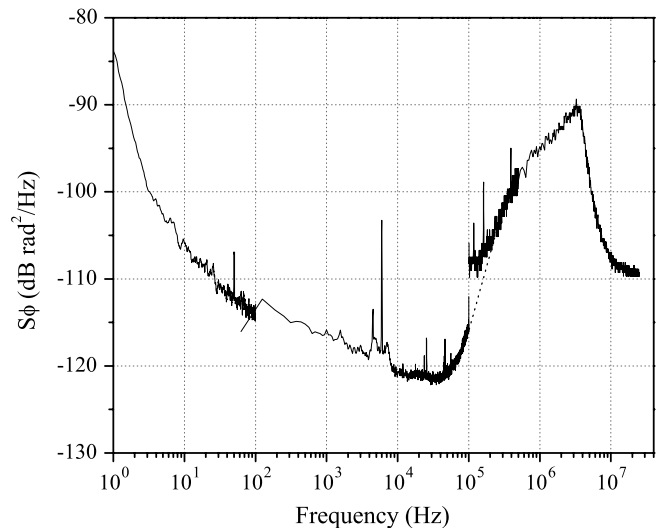
FIGURE 5 Power spectral density of laser phase noise. The measurement is performed by comparing the laser phase with respect to the reference oscillator, with a FFT analyzer below 100 kHz, and with a spectrum analyzer above. Note that the intrinsic phase noise of our spectrum analyzer is about -110 dB rad 2 /Hz at 100 kHz, which is above the lasers phase noise. The bandwidth of the PLL is 3.5 MHz
