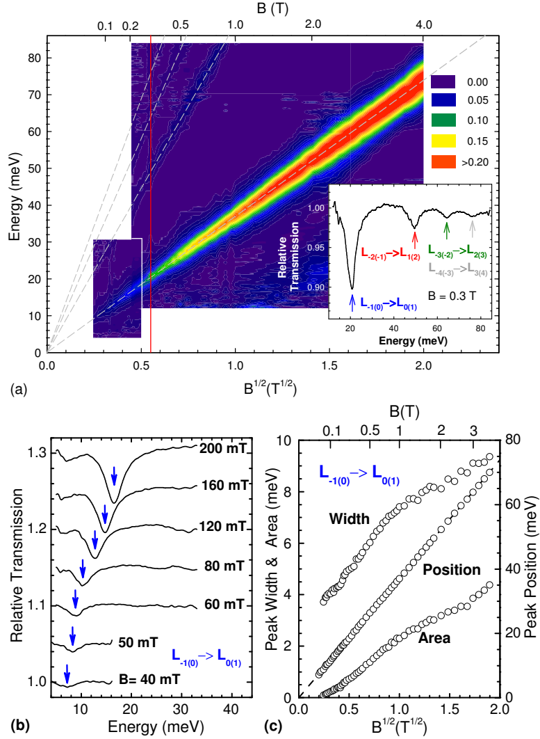
Figure 6.4: Part (a): The FIR transmission \mathcal{T} plotted as -\ln \mathcal{T} as a function of the magnetic field at T = 2.0 K. The dashed lines denote the expected transitions for \tilde{c} = 1.02 \times 10^6 m.s -1 . The inset shows the transmission spectrum at B = 0.3 T. Part (b): FIR transmission taken at T = 2 K in low magnetic fields. Successive spectra are shifted vertically by 0.05. The part (c) shows the peak position, width and area for the L_{-1(0)} \rightarrow L_{0(1)} transition. The dashed line in part (c) is a least squares fit to the peak positions. The measurement was performed on multilayered epitaxial graphene on SiC [130].
