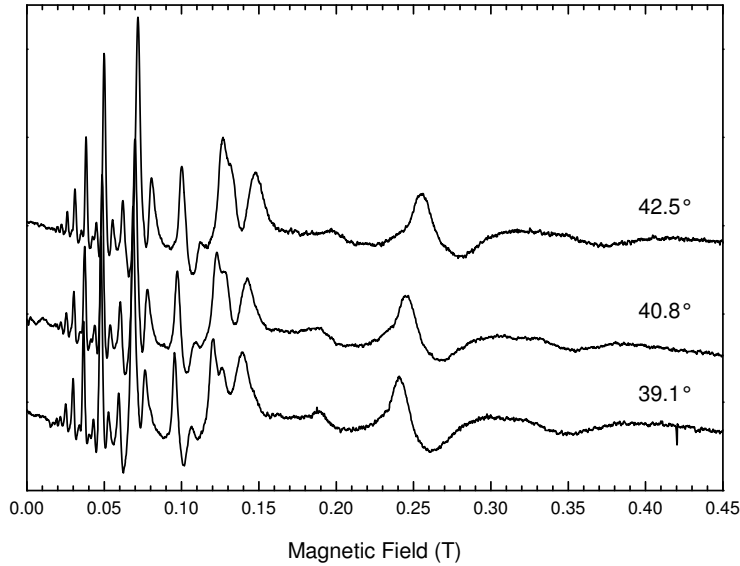
Figure 3.8: . Zoom of single crystal cyclotron resonances of natural graphite at 190 GHz (0.8 meV) and 5 K in the 40^\circ region. The angles were varied in small steps ( 1.7^\circ ) due to the pronounced orientation effect, illustrating the high anisotropy of the system. The measurements was performed with the rotating sample holder (Fig. 3.5c).
