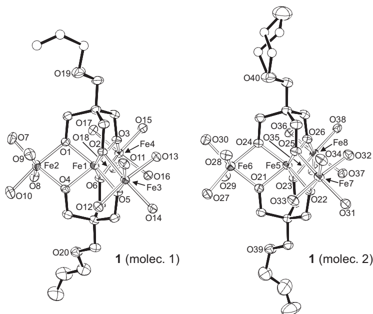
Figure 5.4: ORTEP of the two crystallographically-independent molecules in crystal 1 ( \Lambda isomers). One alkyl chain in molecule 2 is distorted over two approximately equally populated positions. Thermal ellipsoids are drawn at 50% probability. All hydrogen and carbon atoms of dpm^- ligands have been omitted for clarity. The dpm^- is the anion of dipivaloylmethane. Picture taken from Ref. [90] and reprinted with kind permission of A. Cornia.
