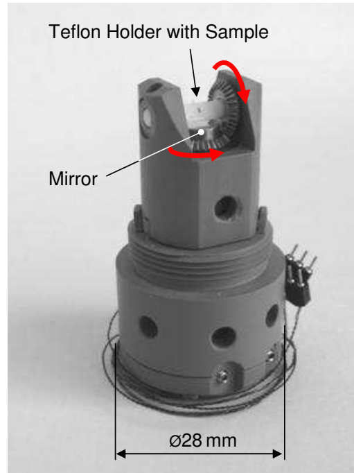
Figure 4.9: Photograph of the rotating holder used for orientation studies of single crystals. The system relies on a rotating piezoelectric nanopositioner ANRv50 (Attocube systems AG) with a resistive encoder allowing an absolute measurement of the angle, hidden in the Torlon housing. The calibrated encoder enables the direct measurement of the position in the range 0^\circ - 337^\circ with position reliability of less than 1^\circ , due to the used mechanical gear.
