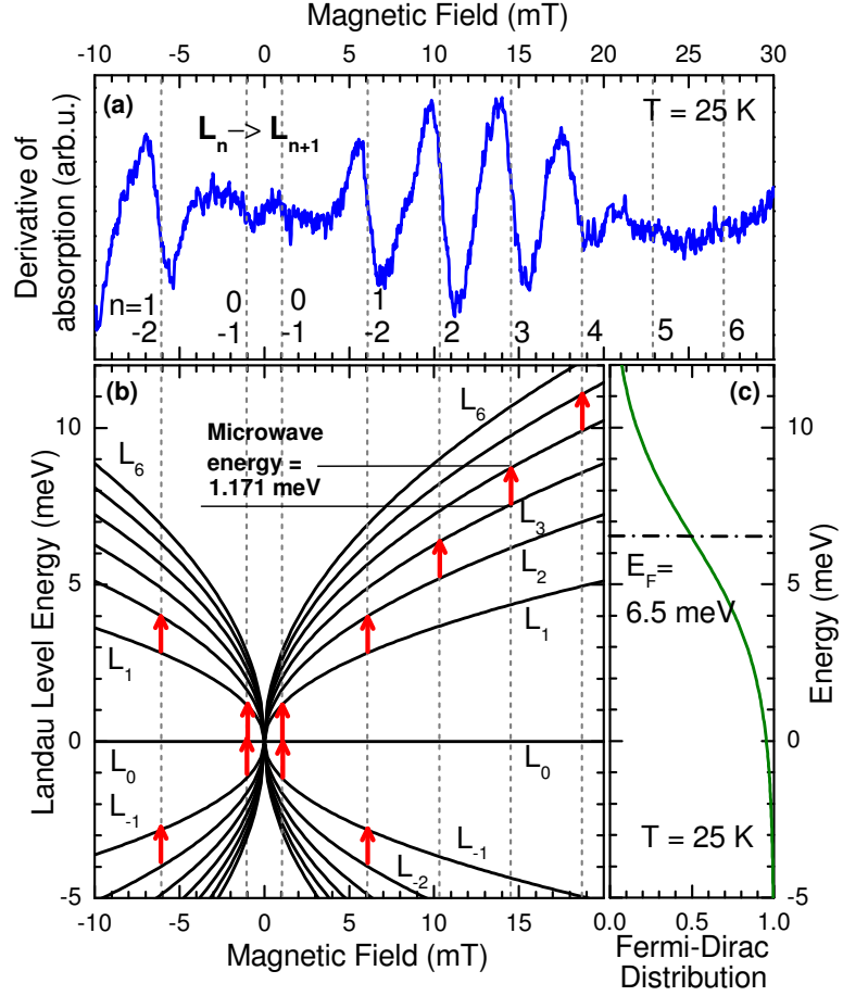
Figure 6.8: Magneto-absorption spectrum (after removing a weak linear background seen in the raw data of Fig. 6.7) measured at T = 25\text{ K} and MW frequency \hbar\omega = 1.171\text{ meV} (230 GHz) (a) in comparison with the LL fan chart (b), where the observed CR transitions are shown by arrows. The occupation of individual LLs is given by the Fermi-Dirac distribution plotted in the part (c). For simplicity, we considered only n -type doping with E_F = 6.5\text{ meV} . The dashed lines show positions of resonances assuming \tilde{c} = 1.00 \times 10^6\text{ m.s}^{-1} .
