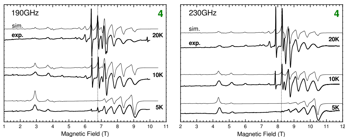
Figure 5.9: Experimental HF-EPR spectra of the powdered sample 4 taken at 190 and 230 GHz at three temperatures (bold lines) superimposed by simulated spectra (narrow line). The parameters used for simulation are given in Table 5.1. The vertical dashed lines in the graphs indicate the central resonance field at 8.21 T (230 GHz) and 6.79 T (190 GHz).
