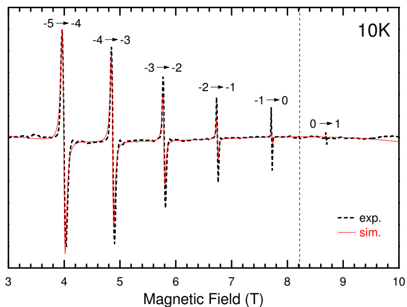
Figure 5.12: HF-EPR spectra of the single crystal of sample 2 with the easy-axis aligned in the direction of the applied magnetic field B (dash line). The red line represent the results of the simulation. The experimental spectrum was simulated with the values D = -0.4472 \text{ cm}^{-1} , E = 0.0354 \text{ cm}^{-1} , B_4^0 = 1.4 \cdot 10^{-5} \text{ cm}^{-1} and B_4^3 = -2.20 \cdot 10^{-3} \text{ cm}^{-1} of the spin Hamiltonian found by the simulation of the single crystal study (Fig. 5.14). The paramagnetic transitions M_S \rightarrow M_S + 1 are indicated in the picture and the dashed line indicates the central resonance field (8.21 T). The spectrum was taken with a non-resonant cavity of the HF-EPR spectrometer in QO configuration at 230 GHz and 10 K.
