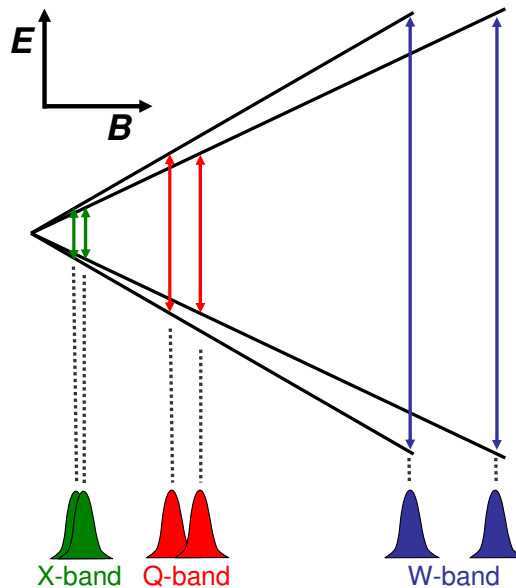
Figure 1.1: Two species of different g -values are very difficult to distinguish at the X-band frequency. The situation gets better for the Q-band frequency where we can already see the two lines presented. However, only the lines for the W-band frequency are fully separated. The resolution of a W-band spectrometer can be considered as one order of magnitude higher than that of a X-band spectrometer.
