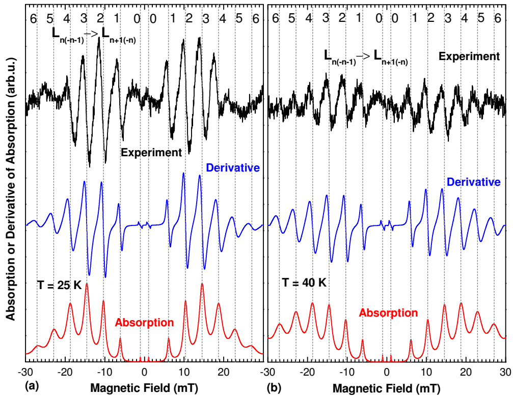
Figure 6.9: Background-removed magneto-absorption spectra from experiment at T = 25 and 40 K (black curves) in comparison to the response at the MW frequency \hbar\omega = 1.171 meV (230 GHz) calculated for parameters \tilde{c} = 1.00 \times 10^6 m.s ^{-1} , \gamma = 35 \mu eV and E_F = 6.5 meV. The dashed lines show the calculated positions of the CR transitions.
