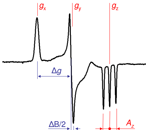
Figure 1.2: Demonstration of the high orientation selectivity, in the picture a spectrum of a radical (TEMPO) taken at 285 GHz (10.2 T). The g -anisotropy as well as the hyperfine interaction is clearly resolved immediately from the spectra. The g -anisotropy will be very difficult to determine from low field X-band spectra with satisfying precision.
