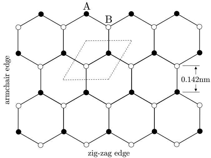
Figure 6.1: Crystallographic structure of graphene consists of two carbon sublattices A (●) and B (○) forming honeycomb lattice. Dashed lines show a unit cell.
