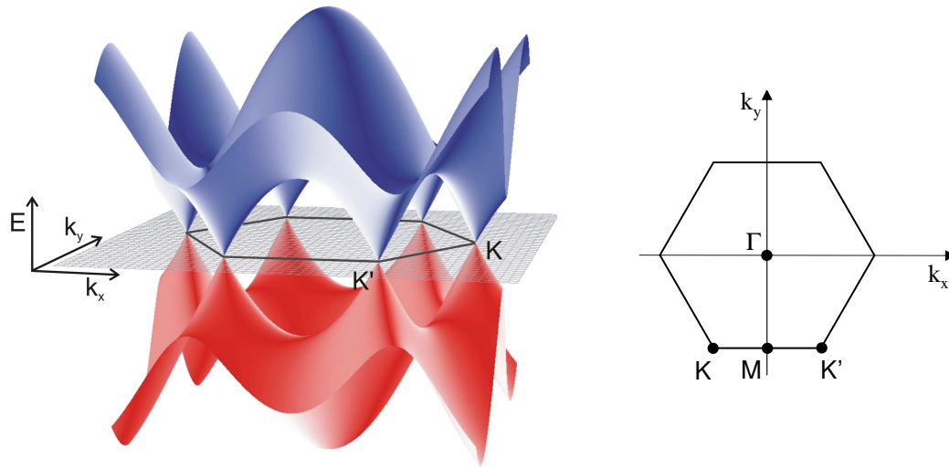
Figure 6.2: Band structure of graphene. The conductance (blue) and valence (red) band touch at K and K' (Dirac) points in momentum space around which the dispersion is linear, creating so-called Dirac cones. Picture reprinted with a kind permission of M. Orlita.
