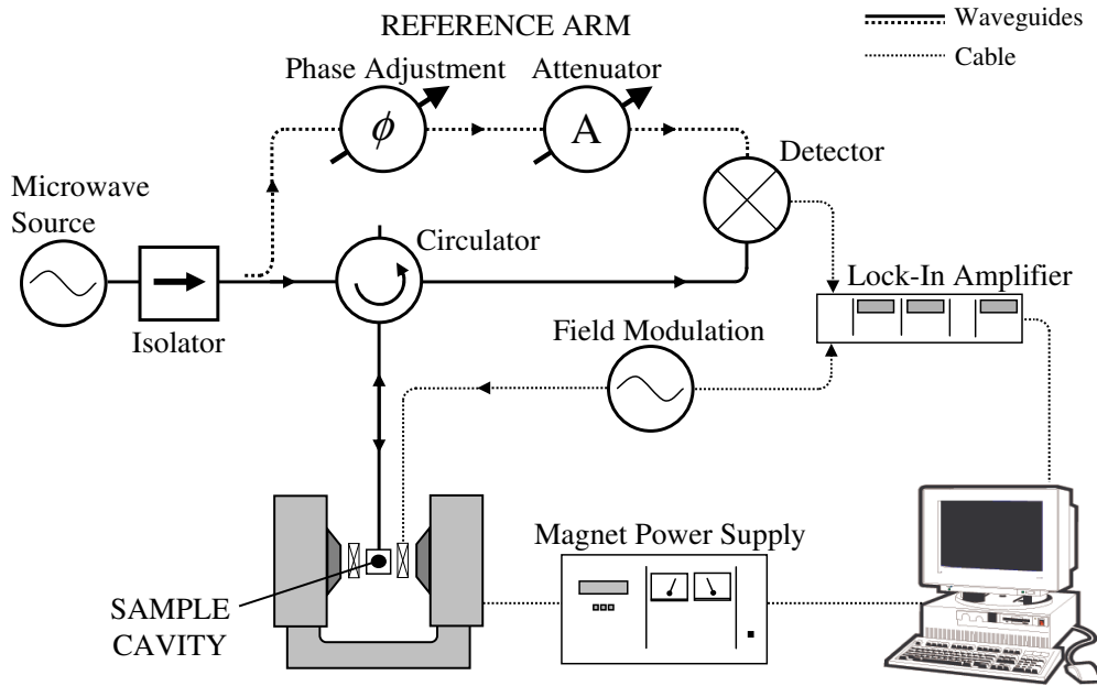
Figure 1.3: Scheme of a standard (X-band) cw-EPR spectrometer with homodyne detector. The MW bridge of the EPR spectrometer utilize single mode rectangular waveguides and other MWs components depicted in the figure. Samples are usually placed into a single mode cavity in the center of a resistive magnet.
