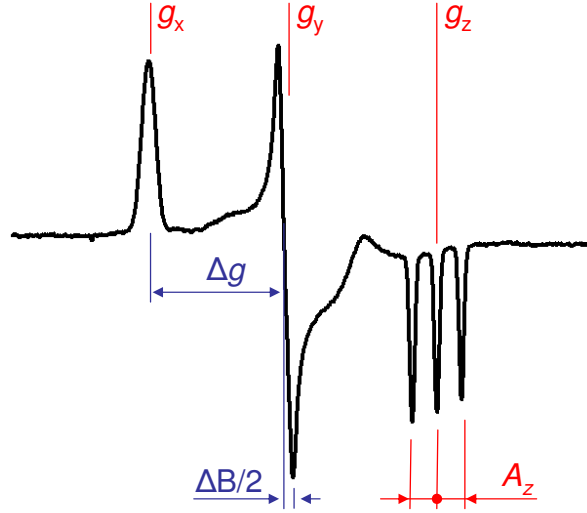
Figure 1.2: Demonstration of the high orientation selectivity, in the picture a spectrum of a radical (TEMPO) taken at 285 GHz (10.2 T). The g -anisotropy as well as the hyperfine interaction is clearly resolved immediately from the spectra. The g -anisotropy will be very difficult to determine from low field X-band spectra with satisfying precision.
