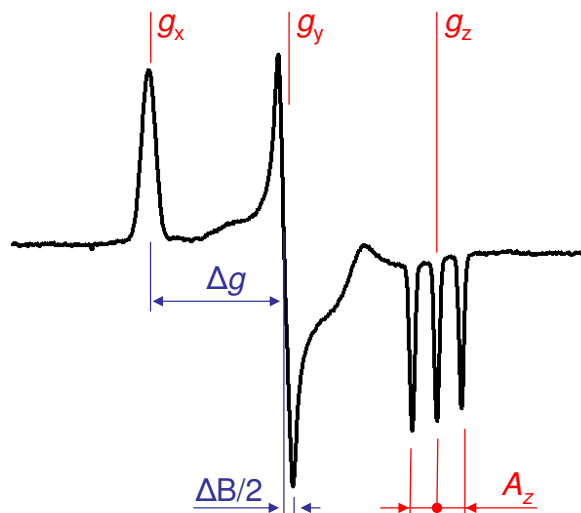
Figure 1.2: Demonstration of the high orientation selectivity, in the picture derivative of the absorption spectrum of a radical (TEMPO) taken at 285 GHz (10.2 T). The g -anisotropy as well as the hyperfine interaction is clearly resolved immediately from the spectra. The g -anisotropy will be very difficult to determine from low field X-band spectra with satisfying precision.
