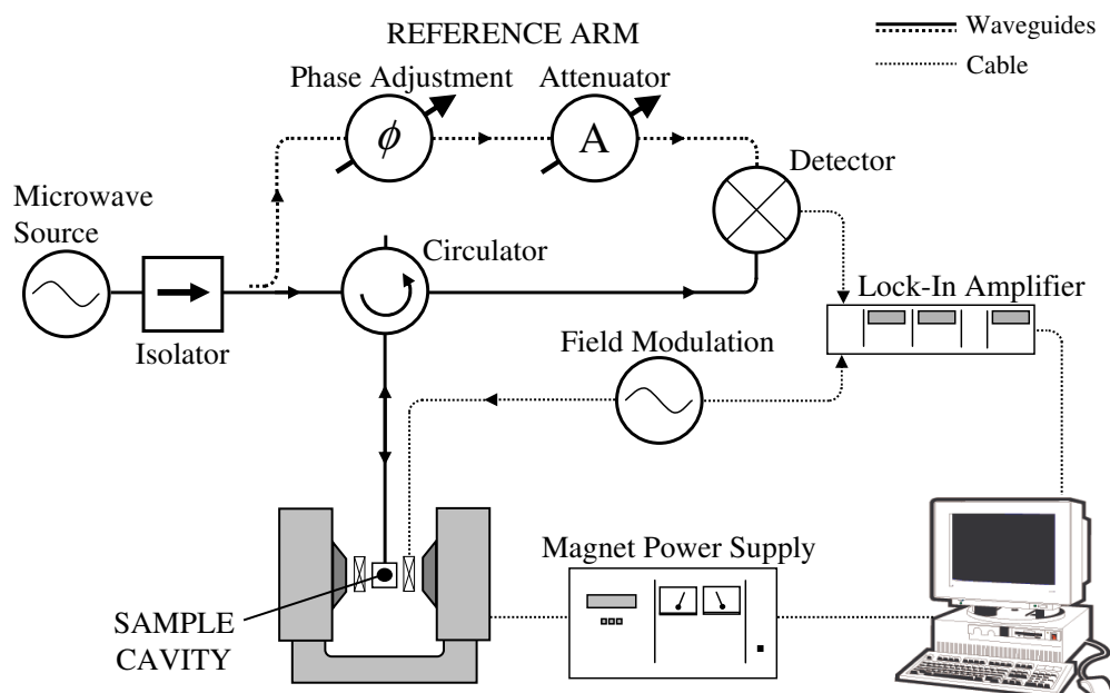
Figure 1.3: Scheme of a standard (X-band) cw-EPR spectrometer with homodyne detector. The MW bridge of the EPR spectrometer utilizes single mode rectangular waveguides and other MW components depicted in the figure. Samples are usually placed into a single mode cavity in the center of a resistive magnet.
