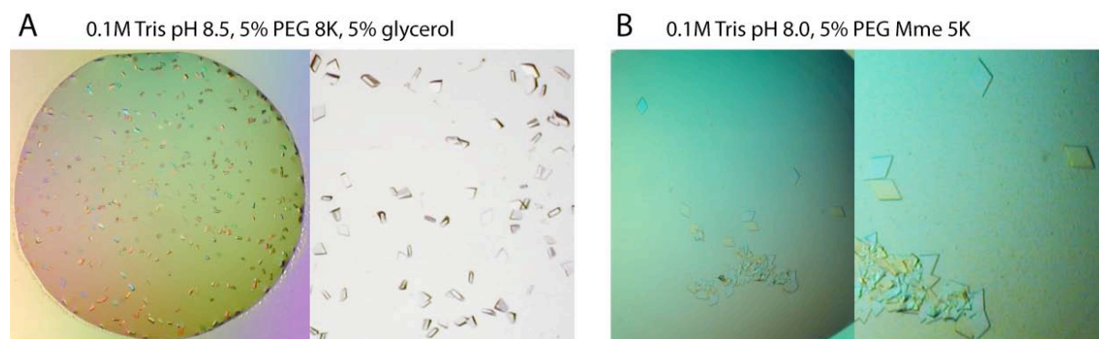
Figure 30. Crystals of AMSH_CT obtained by robot screening can be reproduced by hand.
