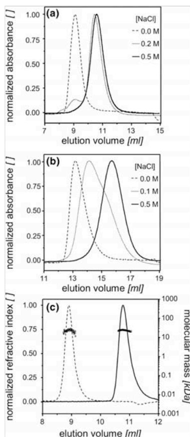
Fig. 1. Enrichment of CHMP3 conformers: Analytical SEC recorded by measuring absorbance at 280 nm (a) on a Superdex™ 75 10/300 GL column with the running buffers 0 HBS (broken line), 200 HBS (dotted line), and 500 HBS (continuous line) as well as (b) on a Superdex™ 200 10/300 GL column with the running buffers 0 HBS (broken line), 100 HBS (dotted line), and 500 HBS (continuous line). A small change in NaCl concentration from 100 HBS to 200 HBS produces a large change in the elution profiles. (c) SEC in combination with refractive index measurement and MALLS performed on a Shodex Protein KW-804 column reveals that CHMP3 in 0 HBS (broken line) and CHMP3 in 500 HBS (continuous line) elute with the observed M_w values of 23.3 \pm 2 kDa (open circle) and 24.1 \pm 0.2 kDa (open square), respectively, which are in agreement with the calculated molecular mass of 24.5 kDa for monomeric CHMP3.
