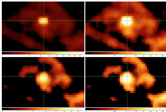
Fig. 9. Reprocessed IRIS images (IRIS) at 60\ \mu\text{m} ( upper panels ) and 100\ \mu\text{m} ( lower panels ). To enhance the suspected extended emission to the south, we present a non-saturated version ( left ) and a saturated one ( right ) for both wavelengths. The field is \sim 65' \times 39' and the green reticles mark the position of RX Lep (north is to the top and east to the left).
