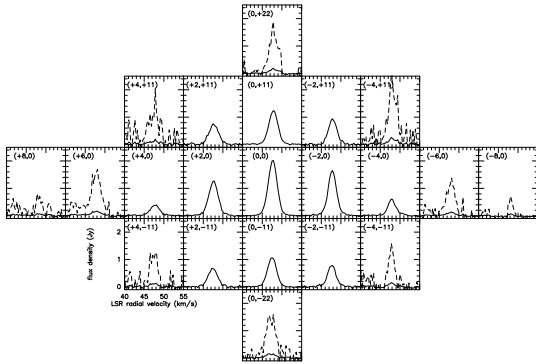
Fig. 2. Map of the 21 cm HI emission of the DDK cloud obtained with the NRT. The central position corresponds to 2MASS 07495348+0430238. The steps are 2' in RA and 11' in Dec; north is up, and east to the left. For the extreme positions, the spectra scaled by a factor 10 are also shown in dashed lines.
