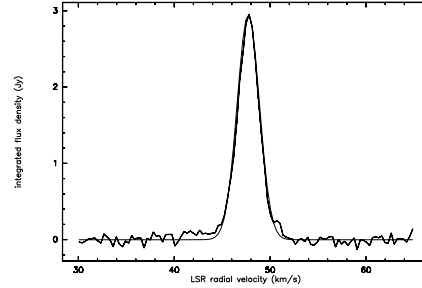
Fig. 3. Integrated HI spectrum of the DDK cloud obtained with the NRT. A fit with one Gaussian ( V_c = 47.74 \text{ km s}^{-1} , FWHM = 2.73 \text{ km s}^{-1} ) is represented by a thin line. An excess of emission can be seen in the wings of the profile.
