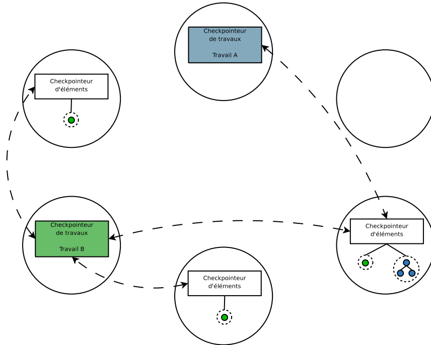
FIG. 3.2 – Architecture de XtremGCP
