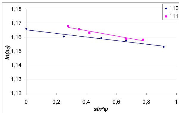
(c) W/W 4/4
