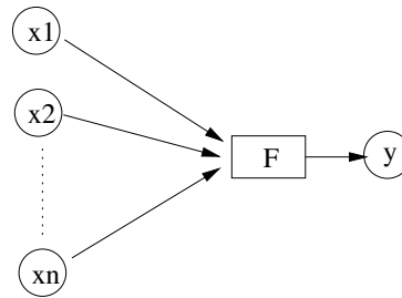
FIG. 2.7 – Neurone formel.
