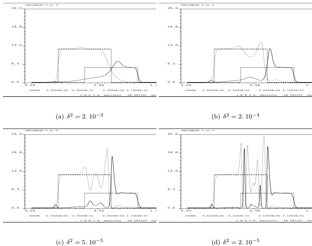
Figure 4.2: Cuts, at a given time, in the y direction and in the middle of the domain \Omega = (0,1)^2 in 2D. The piecewise initial condition is also represented in dashed line. As expected strong oscillations occur with species segregation. These oscillations are stronger when \delta is smaller.
