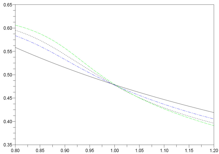
Figure 1.4: Crossing of the Perron and Floquet curves for \psi = \psi_{\text{sin}} (dash dot), \psi_{sq} (dots) and \psi_{pk} (long dash).
