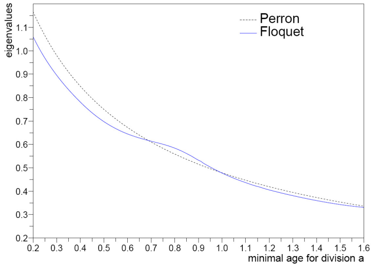
Figure 1.3: Crossing of the Perron and Floquet curves for \psi = \psi_{\text{sin}} .
