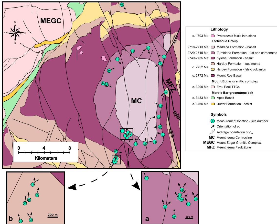
Figure 3.11: Simplified geology of the Meentheena Centrocline compiled from Williams and Bagas (2007a) . Arrows indicate \sigma_H orientations inferred from the data in Tab. 3.1. Large, white arrows are the average orientation of \sigma_H calculated for each of the two insets. Dashed arrows indicate either high uncertainties or direction of stress consistent with Proterozoic faulting.
