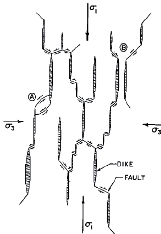
Figure 1.5: Schematic representation of dykes and conjugate fault planes with respect to greatest and least principal stresses \sigma_1 and \sigma_3 . A and B illustrate typical patterns of crack interactions near adjacent dyke tips in homogeneous media. From Pollard [1973].
