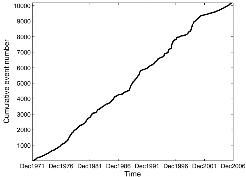
Figure 6.1: Cumulative seismicity ( M \geq M_c = 1.8 ) recorded at Mt. Vesuvius during the period 1972-2006. Completeness of the catalog is constant over time.
