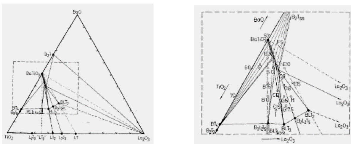
Figure I.13 : diagramme ternaire \text{TiO}_2\text{-La}_2\text{O}_3\text{-BaO} [242].
