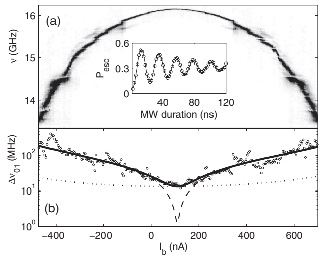
FIG. 3. Camelback phase qubit dynamics. (a) Spectroscopy P_{\text{esc}}(I_b, \nu) at \Phi_{\text{ext}} = -0.503\Phi_0 in the [0\Phi_0] fluxoid state. Dark and bright gray scale correspond to high and small P_{\text{esc}} . P_{\text{esc}} is enhanced when \nu matches \nu_{01} . Inset: Rabi oscillations on the optimal line. (b) Width of the \nu_{01} resonance on a semilog scale. The dashed line is the predicted contribution due to 9 nA rms low-frequency current noise. The dotted line is for 40\mu\Phi_0 rms low-frequency flux noise. The sum of these two contributions, the solid line, accurately reproduces the data (symbols).
