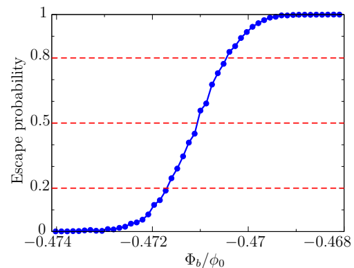
Figure 3.19: Escape probability as a function of the flux bias.
