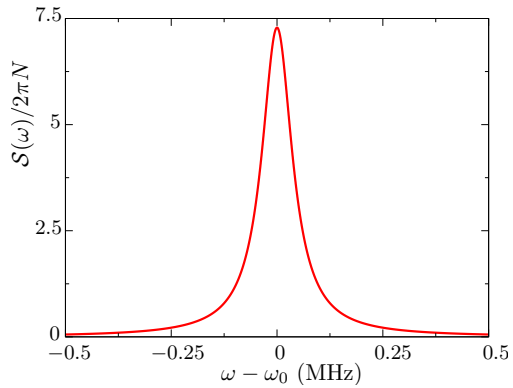
Figure 4.7: Spectrum at the resonance. The linewidth is found to be about 90 kHz.
