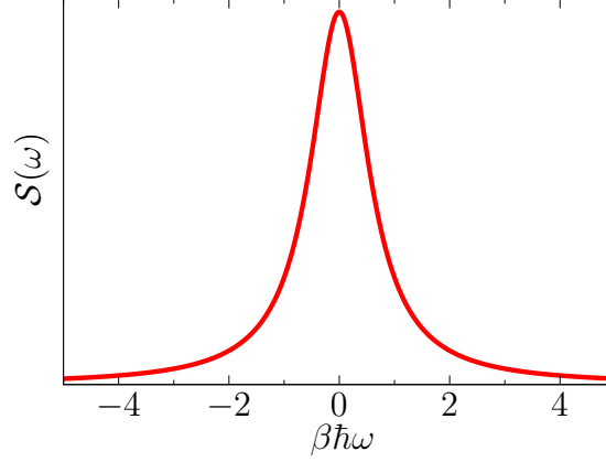
Figure 6.1: Real part of the symmetrized voltage spectrum \mathcal{S}(\beta\hbar\omega) from an extended analysis of Chap. 2 with \beta U_0 = 0.1 , \beta\hbar\omega_c = 10 , g = 0.1 , I_b = V_c/R and s_{-1} = -s_0 .
