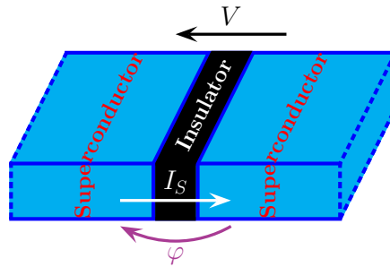
Figure 1.4: A schematic representation of a superconducting Josephson junction. Two superconducting electrodes are connected to each other via an insulating layer.
