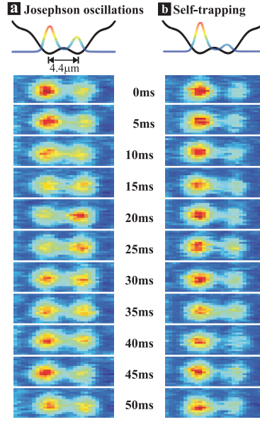
Figure 1.13: Direct observation of tunneling in a single Bose Josephson junction [40]. Left : time-resolved Josephson oscillations. Right : macroscopic quantum self-trapping.
