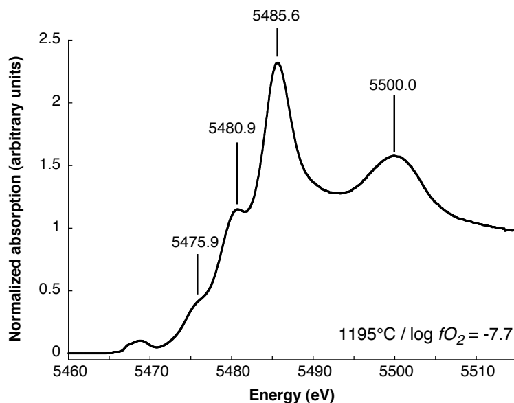
Figure 5.21: V K -edge HERFD-XAS spectrum of the ( T = 1195^\circ\text{C} , \log f_{\text{O}_2} = -7.7 ) sample, illustrating the features observed in the six synthesized samples containing magnetite.
