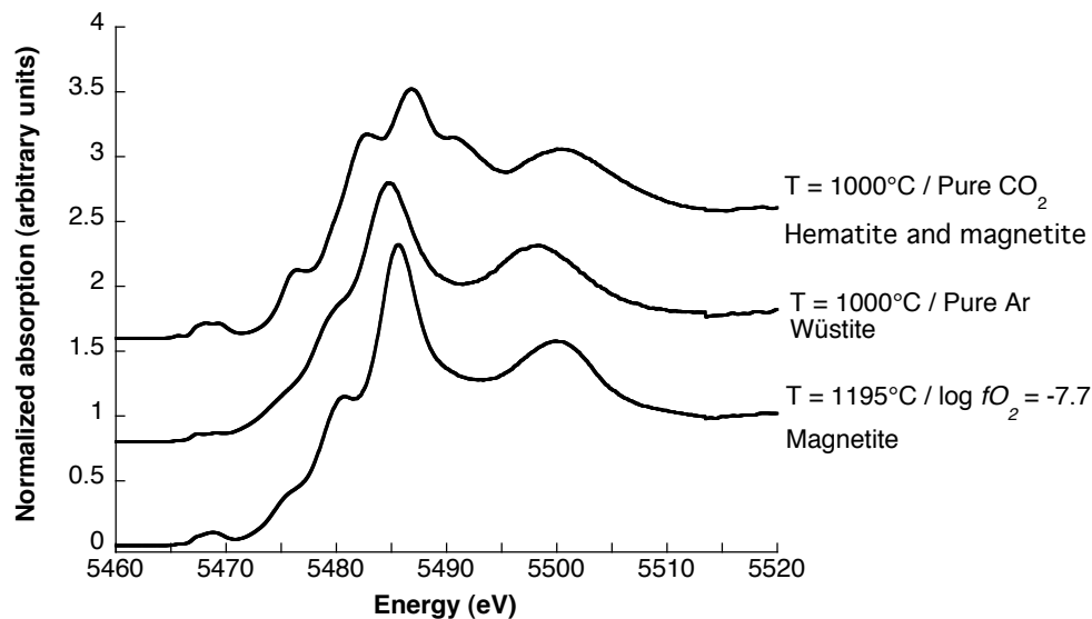
Figure 5.20: V K -edge HERFD-XAS spectra of the three samples containing respectively magnetite ( T = 1195^\circ\text{C} , \log f_{\text{O}_2} = -7.7 ), wüstite ( T = 1000^\circ\text{C} , pure Ar) and hematite + magnetite ( T = 1000^\circ\text{C} , pure \text{CO}_2 ).
