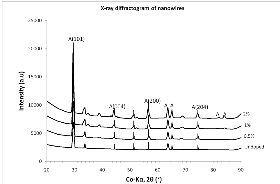
Figure 3. X-Rays Diffractograms of undoped and doped samples
