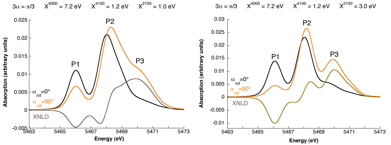
Figure 3.12: The spectra of the experimental \alpha_{rot} = 0^\circ and \alpha_{rot} = 90^\circ orientations for two sets of crystal-field parameters, illustrating the influence of the X^{2100} parameter on the spectra, for X^{4000} = 7.2 eV, X^{4100} = 1.2 eV and 3\alpha = \pi/3 .
