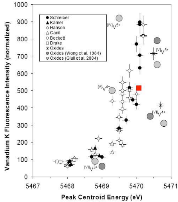
Figure 8. Pre-edge intensity vs. peak energy (after Sutton et al., 2005). The parameters measured on the \text{V} -doped sample are characteristic of \text{V}^{4+} in octahedral coordination.
