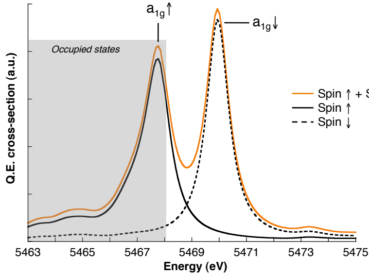
Figure 3.8: Calculated electric quadrupole cross-section with the spin-polarization, for the (\hat{\epsilon} = [-\frac{1}{\sqrt{3}}, \frac{1}{\sqrt{3}}, \frac{1}{\sqrt{3}}], \hat{\mathbf{k}} = [-\frac{1}{\sqrt{3}}, \frac{1}{\sqrt{3}}, \frac{1}{\sqrt{3}}]) configuration.
