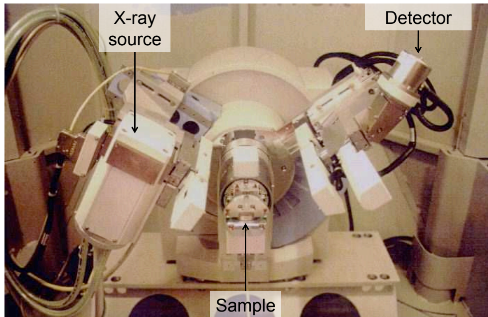
Figure 1.9: Picture of the \theta - \theta diffractometer. The sample is kept fixed while the X-rays source and the detector rotate by an angle \theta .
