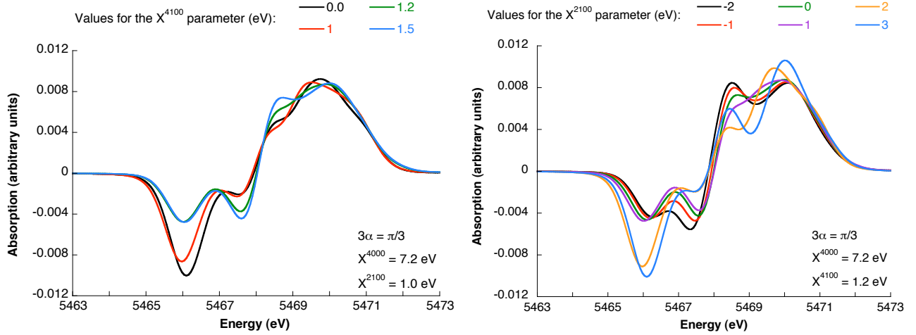
Figure 3.11: The influence of the X^{4100} left and X^{2100} right parameters on the dichroic signal for a fixed value of X^{4000} and 3\alpha parameters.
