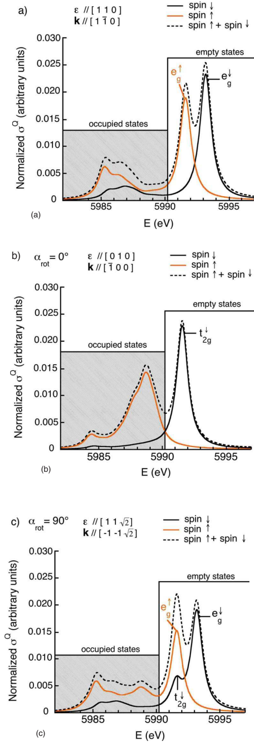
FIG. 5. (Color online) Electric quadrupole transitions calculated for site A using spin polarization. The upper panel (a) presents the spectrum calculated for (\hat{\epsilon} = [\frac{1}{\sqrt{2}}, \frac{1}{\sqrt{2}}, 0], \hat{\mathbf{k}} = [\frac{1}{\sqrt{2}}, -\frac{1}{\sqrt{2}}, 0]) . The middle panel (b) presents the spectrum calculated for \alpha_{\text{rot}} = 0^\circ ( \hat{\epsilon} = [010], \hat{\mathbf{k}} = [\bar{1}00] ). Lower panel (c) presents the spectrum calculated for \alpha_{\text{rot}} = 90^\circ ( \hat{\epsilon} = [\frac{1}{2}, \frac{1}{2}, \frac{1}{\sqrt{2}}], \hat{\mathbf{k}} = [-\frac{1}{2}, -\frac{1}{2}, \frac{1}{\sqrt{2}}] ). For each configuration, the respective contributions of the two spins are plotted (black solid line for spin down, orange solid line for spin up), as well as the sum (dashed line). The Fermi level is located approximately around 5990 eV.
