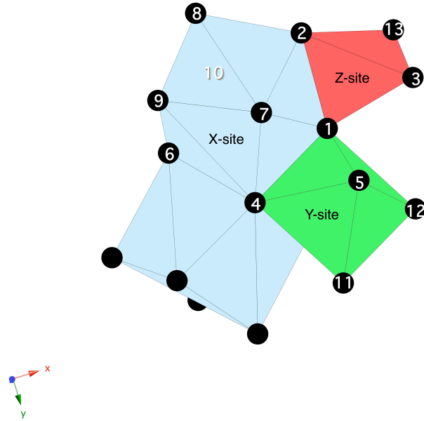
Figure 2: Portion of the tsavorite garnet structure, with X=\text{Ca}^{2+} , Y=\text{Al}^{3+} and \text{V}^{3+} , and Z=\text{Si}^{4+} . The O atoms are labelled according to Novak and Gibbs (1971). The figure is taken from Juhin et al. (2008a).
