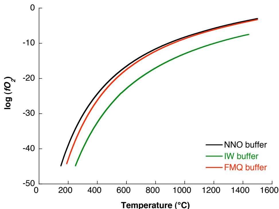
Figure 5.5: Evolution of the oxygen fugacity as a function of the temperature for the Faylaite-Magnetite-Quartz (FMQ), Iron-Wüstite (IW) and Nickel-Nickel Oxide (NNO) buffers
