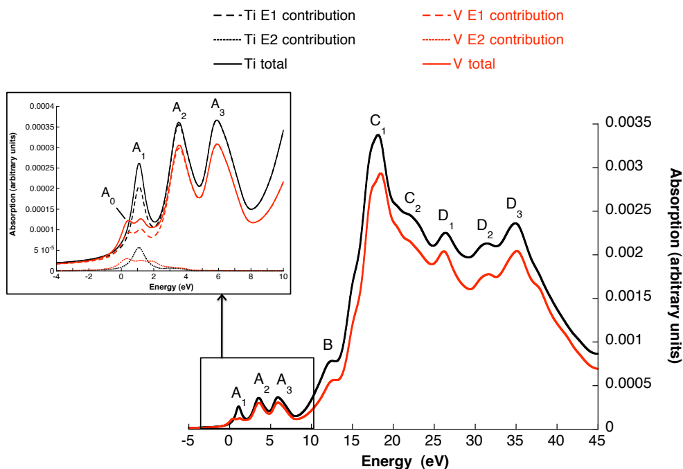
Figure 4.11: Comparison between the isotropic calculated spectra of anatase at the V (red) and Ti (black) K -edge. The pre-edges are displayed in the inset.
