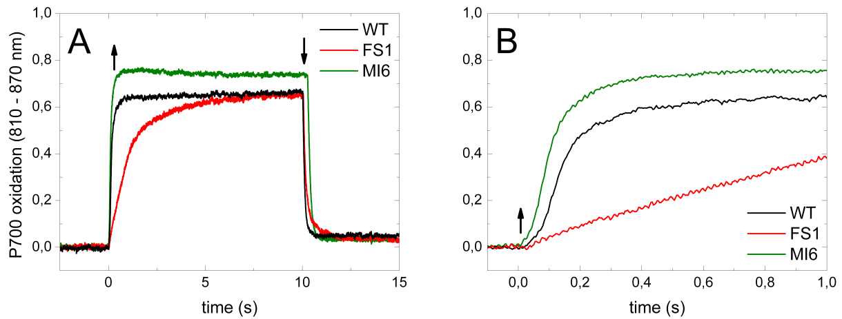
Figure 3.8 P700 oxidation and reduction kinetics in low CO 2 of WT (black), FS1 (red) and MI6 (green) mutant strains.
