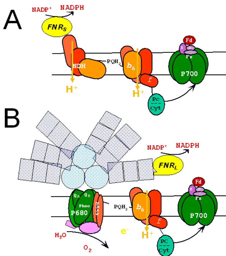
Figure 3.12 Representation of the possible association of FNR S with NDH-1 (A) and the known association of FNR L with PBS (B).
