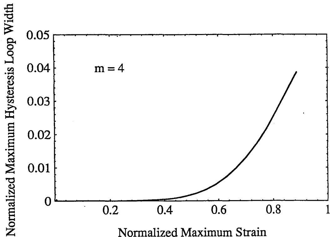
Fig. 7. – Normalized maximum hysteresis loop width, \delta \bar{\epsilon} E_F / S_c as a function of maximum normalized strain, \bar{\epsilon} E_F / S_c .
