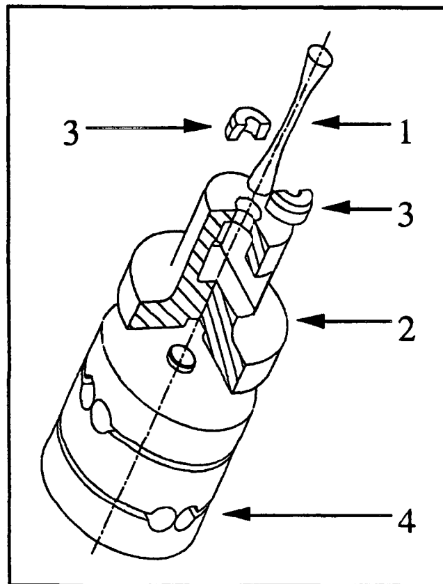
FIG. 1—The gripping system for tensile tests [1] (1- specimen, 2- grip, 3- half shells, 4- elastic joint).
