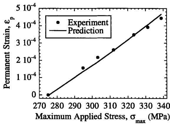
Figure 6. Permanent strain \epsilon_p versus maximum applied stress \sigma_{max} for a SiC/SiC composite.
