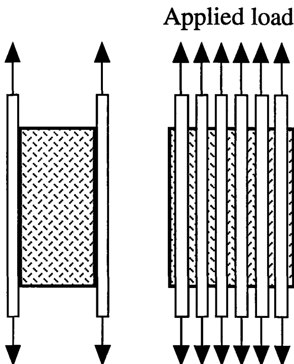
Figure 8. Schematic of an ID2 specimen.
