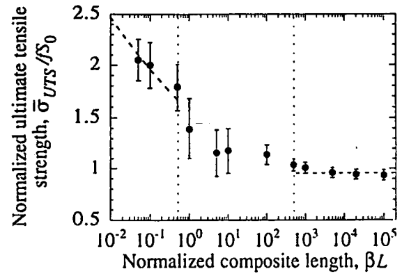
Fig. 4. Normalized ultimate tensile strength of an E Glass/Epoxy composite as a function of normalized composite length ( \beta = 10 \text{ mm}^{-1} , fS_0 = 900 \text{ MPa} , L_0 = 10 \text{ mm} , m = 10 , \mu = 0.9 , \tau_d = 80 \text{ MPa} , R = 5.5 \text{ }\mu\text{m} ).
