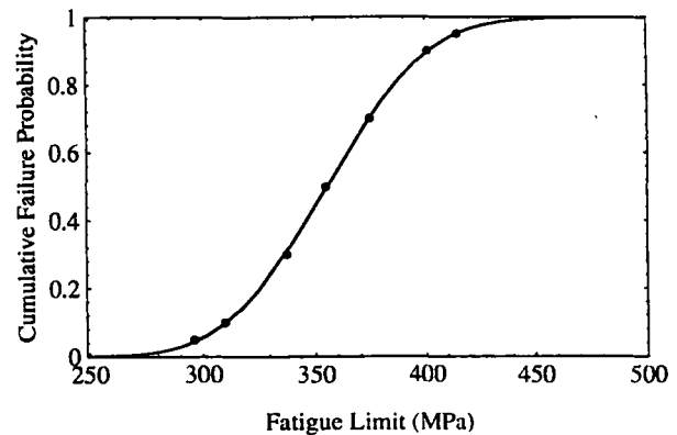
Fig. 5. Experiments and predictions of the fatigue limits for different cumulative failure probabilities ( \alpha = 1.75 , \beta = 17.5 , V/V_0 = 112 , S_u = 520 MPa, k = 1/3 ).
