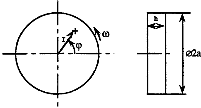
FIGURE 2. THE GEOMETRY OF THE CIRCULAR DISC ( a = .3 m, h = .01 m).
