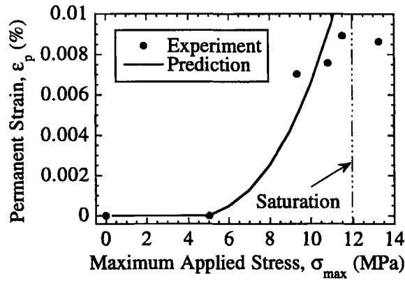
Figure 12. Permanent strain \epsilon_p versus maximum applied stress \sigma_{\max} for two ID2 concrete specimens ( f_{sf} = 0\% ).
