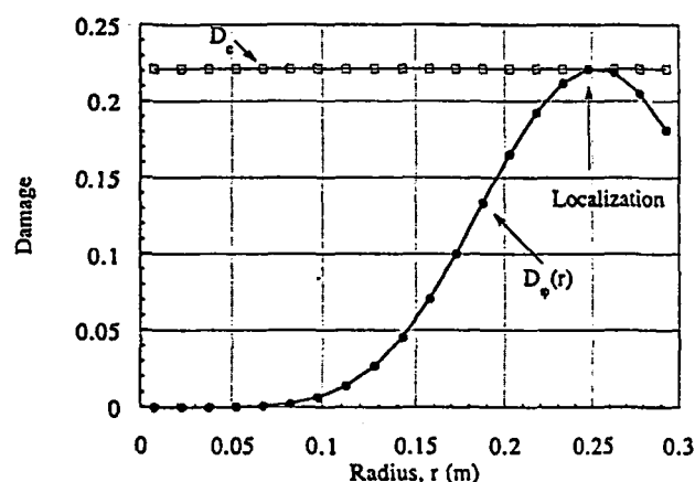
Fig. 9. Damage variable D_{\phi}(r) as a function of the radius intersecting (see the arrow) the critical damage value at localization ( \rho\omega^2 = 0.59 \cdot 10^{10} \text{ kg m}^{-3} \text{ s}^{-2} ) for a fully coupled computation applied to the disk with model No. 0.
