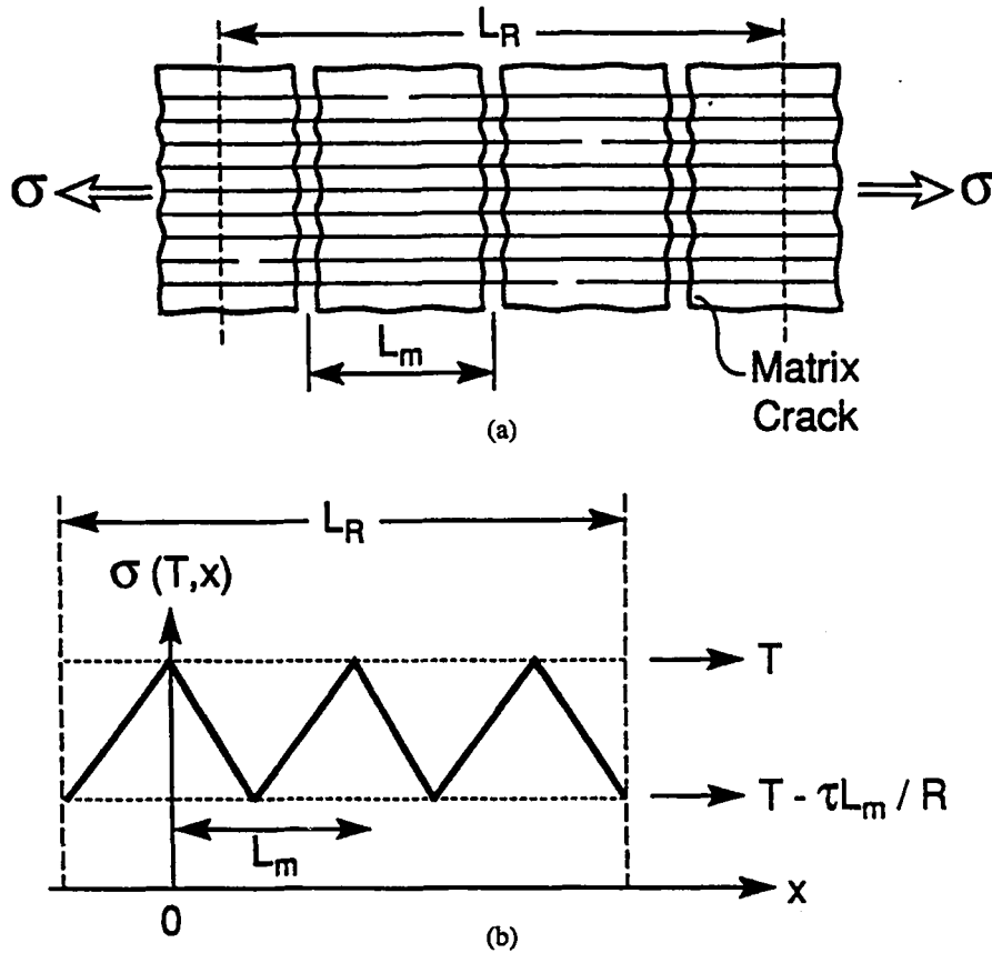
Fig. 1 a. – Depiction of the recovery length L_R when the density of matrix cracks (characterized by L_m ) reaches saturation.
