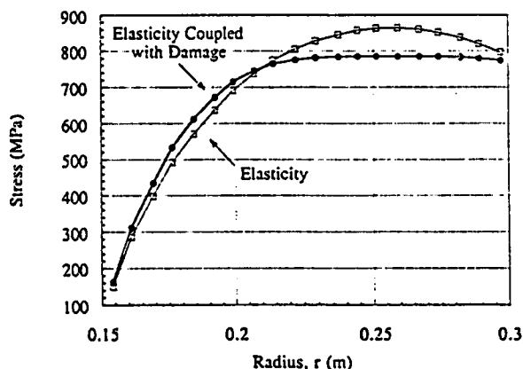
Fig. 5. Hoop stress \sigma_{\varphi\varphi}(r) as a function of the radius obtained by fully coupled computation and a decoupled computation at localization ( \rho\omega^2 = 2.26 \cdot 10^{10} \text{ kg m}^{-3} \text{ s}^{-2} ) for the ring with model No. 1. Note the stress redistribution.
