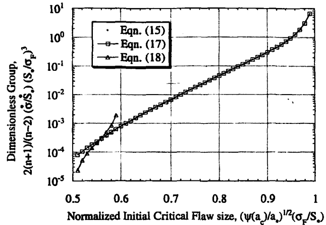
Fig. 2 Comparison of the evolution of a dimensionless group, 2(n+1)/(n-2)(\sigma/S_*)(S_*/\sigma_F)^3 , as a function of normalized initial critical flaw size, (\psi(a_c)/a_*)^{1/2}(\sigma_F/S_*) , by using Eqs. (15), (17), and (18). The parameter n is equal to 16, and the energy release rate ratio k is equal to 0.5.
