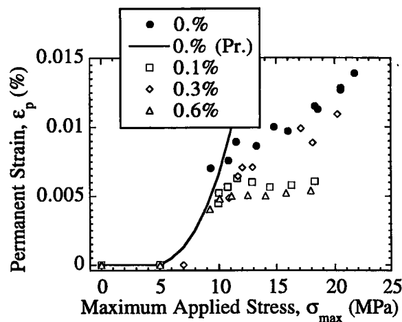
Figure 16. Permanent strain \epsilon_p versus maximum applied stress \sigma_{max} for ID2 specimens f_{sf} = 0., 0.1, 0.3 and 0.6\% . The symbols are experimental data and the solid line is the prediction when f_{sf} = 0\% .
