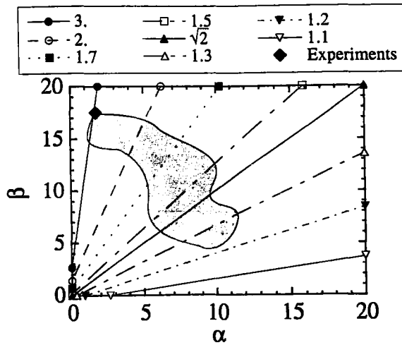
Fig. 10. Fatigue gfailure map giving the boundary of the monotonic failure and no-failure zones as a function of the parameters \alpha and \beta when P_{F0}=50\% for different normalized stress levels \sigma_g(R)/S_{th} or \sigma_g(R)/S_{th} .
