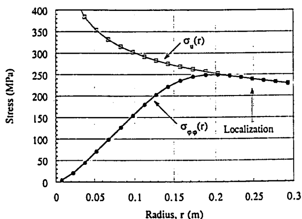
Fig. 7a. Hoop stress \sigma_{\phi\phi}(r) as a function of the radius intersecting (see the arrow) the r -dependent ultimate tensile strength \sigma_u(r) at localization ( \rho\omega^2 = 0.59 \cdot 10^{10} \text{ kg m}^{-3} \text{ s}^{-2} ) for a fully coupled computation applied to the disk with model No. 0. Note the r -dependence of the ultimate tensile strength.
