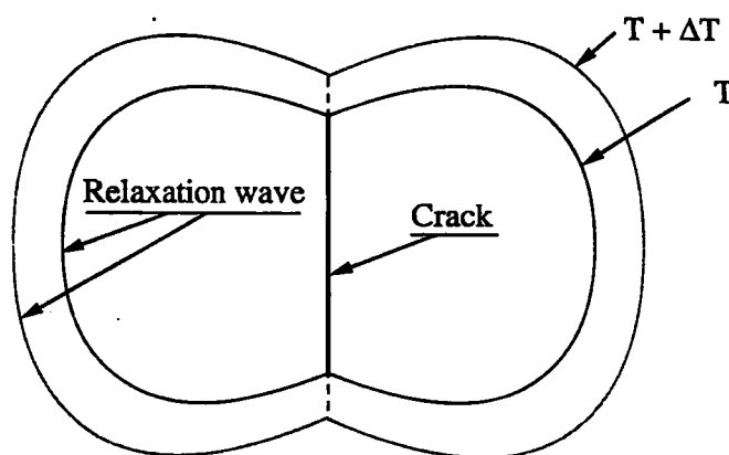
Fig. 1. - Relaxation around a propagating crack at time T and T + \Delta T .
