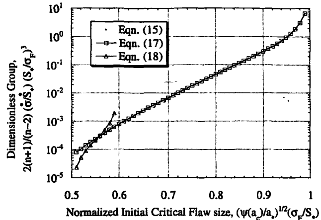
Fig. 2 Comparison of the evolution of a dimensionless group, 2(n + 1)/(n - 2)(\sigma_F/S_*)(S_*/\sigma_F)^3 , as a function of normalized initial critical flaw size, (\psi(a_c)/a_*)^{1/2}(\sigma_F/S_*) , by using Eqs. (15), (17), and (18). The parameter n is equal to 16, and the energy release rate ratio k is equal to 0.5.
