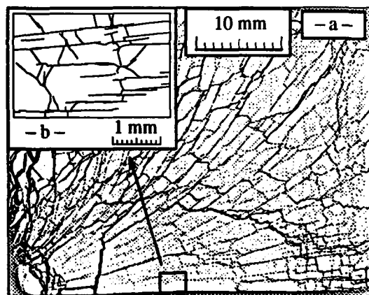
FIGURE 2. a-Half top view of tile impacted at a velocity of 330 m/s. b-The magnification shows many short radial cracks linked by short circumferential ones.
