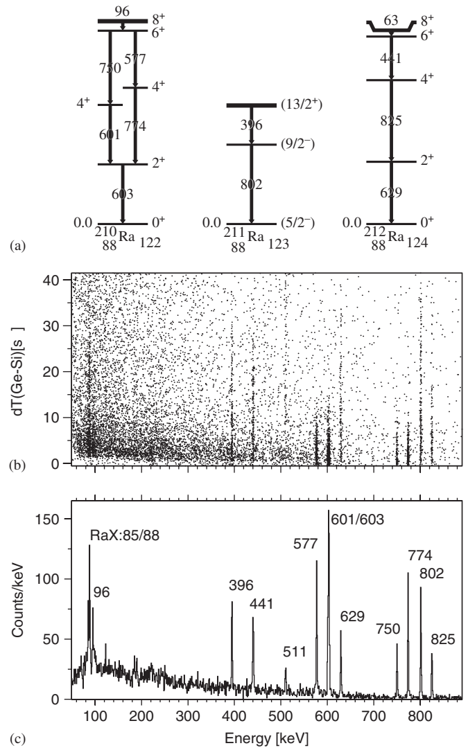
Fig. 6. (a) Partial level schemes (taken from Refs. [38–41]) below the isomeric states in the radium isotopes populated via the ^{174}\text{Yb}(^{40}\text{Ar}, x\text{n})^{214-x}\text{Ra} reaction and transported to the focal plane of VASSILISSA. (b) The time difference between recoil and \gamma -ray detection as a function of measured \gamma -ray energy is plotted on an event-by-event basis. (c) Delayed \gamma -ray transitions observed within 40\mu s after the recoil was detected.
