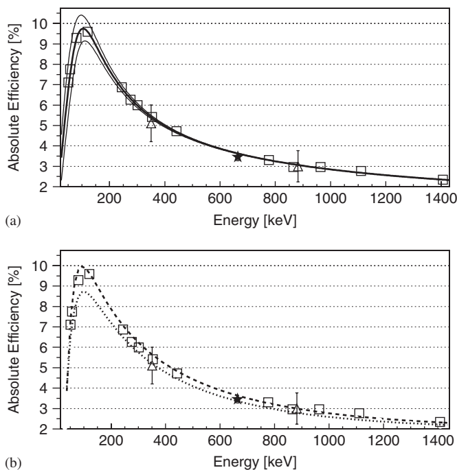
Fig. 3. Absolute efficiency curve for the 7 Ge detectors. \square , measured using ^{133}\text{Ba} , ^{152}\text{Eu} and ^{241}\text{Am} sources; \star , measured using \gamma -electron coincidences from the decay of an isomeric state in ^{207}\text{Rn} implanted into the stop detector using the reaction ^{164}\text{Dy}(^{48}\text{Ca}, 5n) ; \Delta , measured using \alpha - \gamma coincidences from the fine-structure decay of ^{211}\text{Bi} [ E_{\gamma} = 351 keV] and ^{217}\text{Th} [ E_{\gamma} = 882 keV]. (a) the bold solid line: fit to the data using the expression \log(\varepsilon) = [(A + Bx_1 + Cx_1^2)^{-G} + (D + Ex_2 + Fx_2^2)^{-G}]^{-1/G} where x_1 = E_{\gamma}/100 and x_2 = E_{\gamma}/1000 ; the thin solid lines represent the error in the fit; (b) dashed line: Geant4 simulated efficiency curve for a point source positioned at the centre of the stop detector; dotted line: Geant4 simulated efficiency curve for a distributed source.
