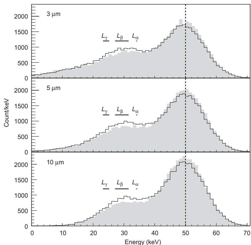
Fig. 12. Same as Fig. 10 with a detector resolution of 15 keV.
