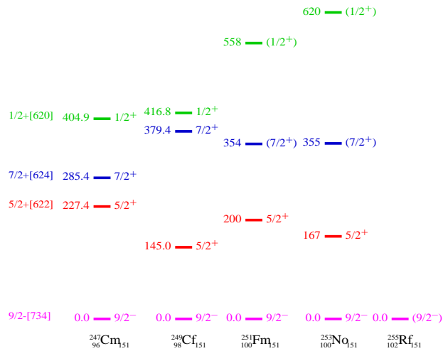
Fig. 5. Systematics of low-lying levels in N = 151 isotones obtained from refs. [26–29] and this work.
