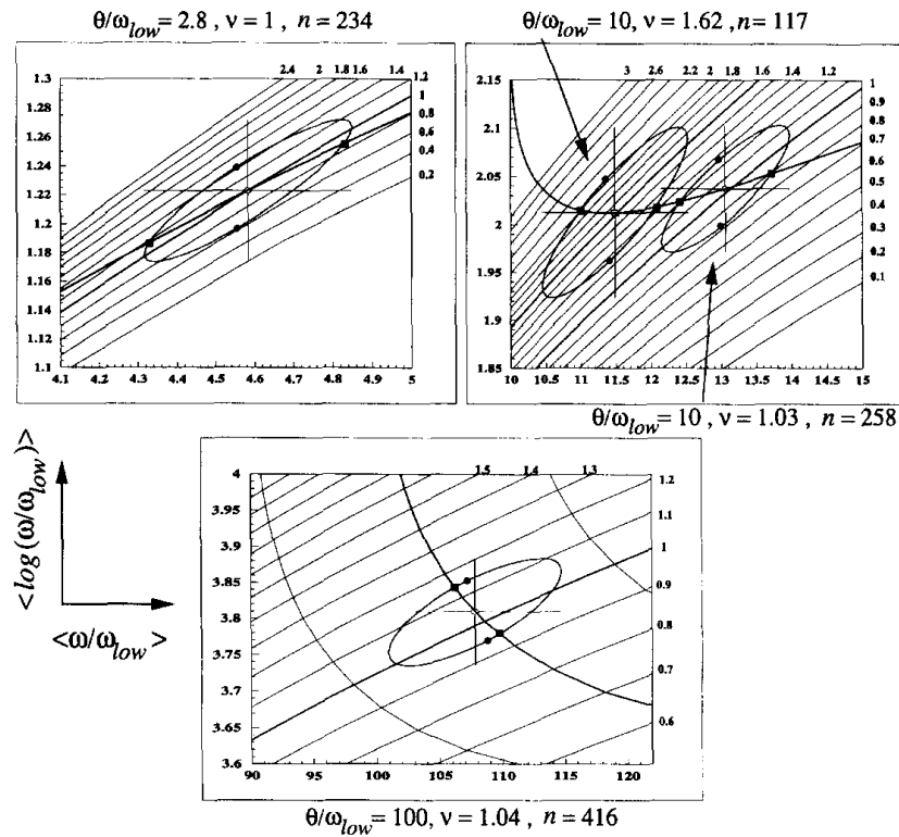
Fig. B.1. Dispersion ellipses are shown, together with the extreme values of \nu on their perimeter (dots), and the intersection with contours of constant \theta (squares), thereby illustrating the different values of the dispersion in \nu one obtains for the whole distribution (dots) and with restriction to fixed \theta (squares). The values of the estimated average relative to the cut-off, the determined number of degrees of freedom \nu , and the sample size in the three panels are taken from the analysis by Garrison [10].
