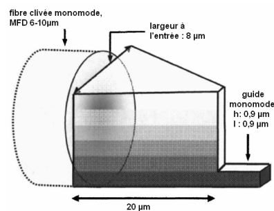
(a) GRIN coupleur, efficacité 61% [22]
