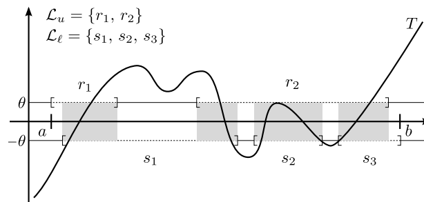
Figure 3.2 : Comment calculer \mathcal{Z}
