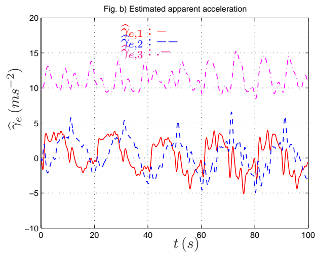
Figure 2.6: Real ( \gamma_e ) and estimated ( \hat{\gamma}_e ) apparent accelerations.
