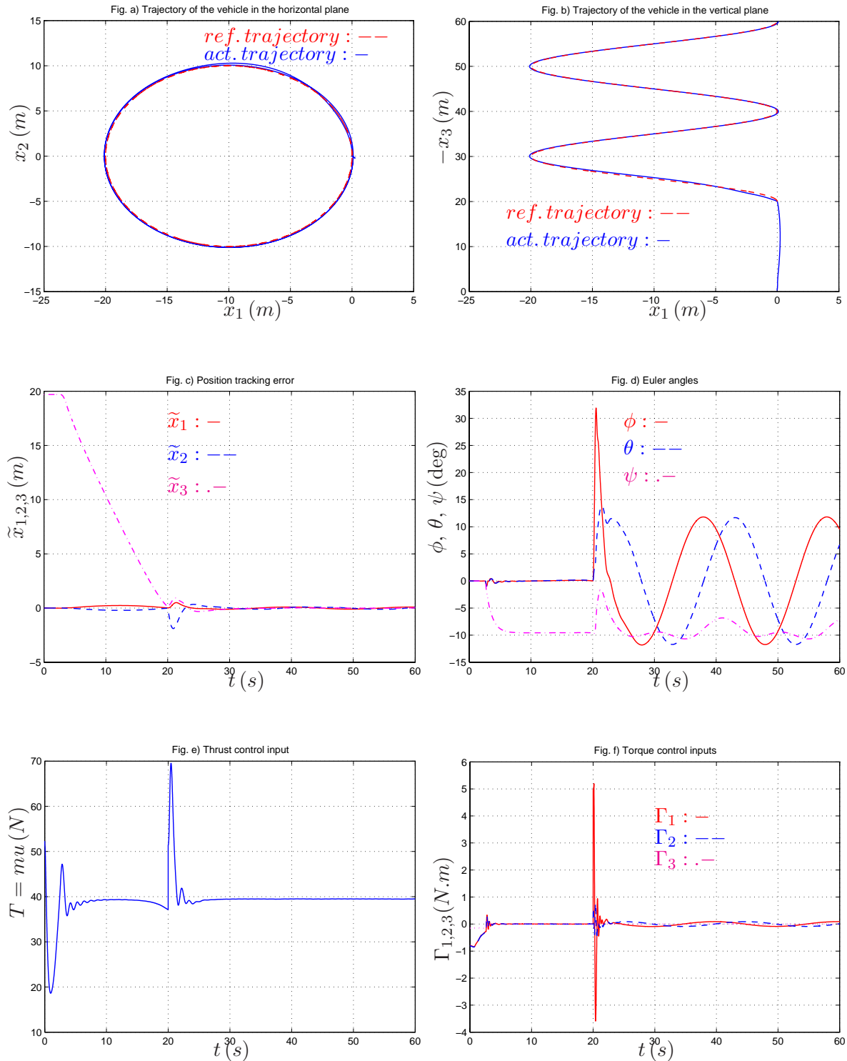
Figure 2.9: Simulation results with the HoverEye simulator. Take-off flight. Ascending reference spiral and vehicle's trajectory in the absence of wind.
