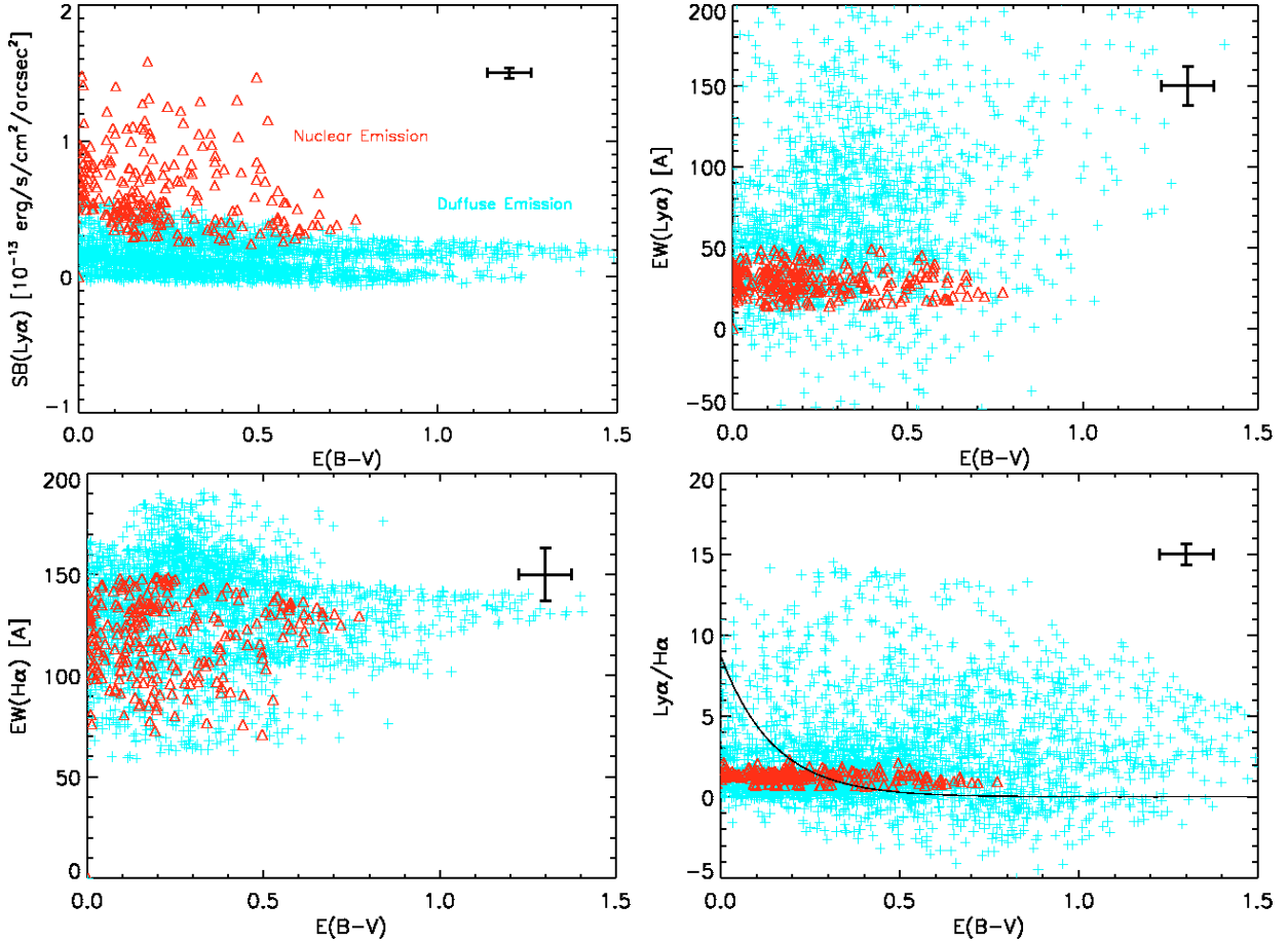
Fig. 6. IRAS 08339+6517 scatter plots. Top-left: Ly \alpha surface brightness vs. E(B - V) . The nuclear Ly \alpha emission component is represented in red, and the diffuse emission component is in cyan. Same color code applied in all the plots. Top-right: Ly \alpha equivalent width vs. E(B - V) . Bottom-left: H \alpha equivalent width vs. E(B - V) . Bottom-right: Ly \alpha /H \alpha ratio vs. E(B - V) . Error bars correspond to the uncertainties estimated in Sect. 2.3.
