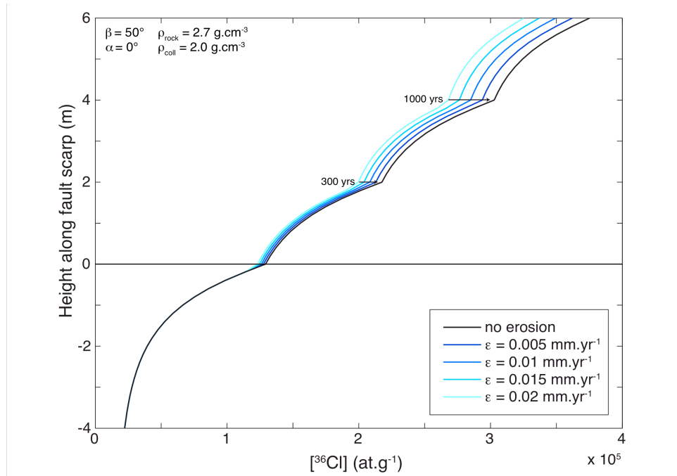
FIG 8: Effect of erosion on the ^{36}\text{Cl} profile resulting in exposed scarp rocks. A reference curve is calculated for no erosion and 3 similar (2 m of on-fault slip), regular (every 2 kyrs) earthquake exhumations. Ages are maximum age differences that are derived between the most extreme curves.
