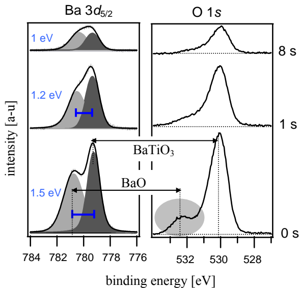
Figure 3.5.8: The Ba 3d_{5/2} and O 1s core levels during Pt deposition of BTO thin film highly oxidized. The Pt deposition time is indicated in second. Energy separation between BaO and bulk components also decreases with Pt deposition as in the case of BTO without apparent BaO bonding (see Fig. 3.5.6).
