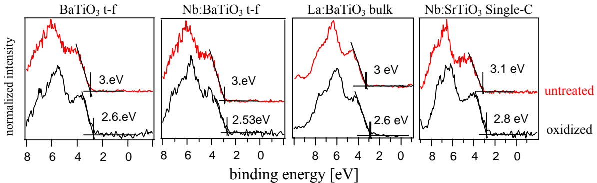
Figure 3.4.6: X-ray valence band spectra for thin films, ceramic, and single crystal used in the present study. Lowering of the Fermi level is evident after oxidation for all these systems.
