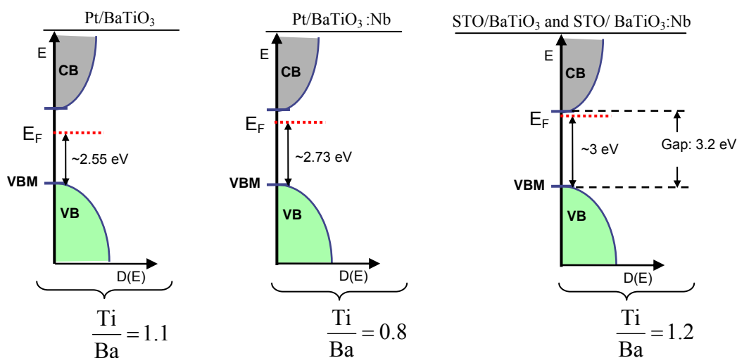
Figure 3.1.1.6: Fermi level position for pure and Nb-doped BTO thin films deposited onto Pt(111) and STO:Nb(100) using the optimised deposition conditions determined in the first paragraph. For Pt/BTO thin film, the E_F values are derived from the previous paragraph. However, Pt/BTO:Nb exhibit higher Fermi level due to doping effect (see III.3.3). For STO:Nb crystal substrates, no change is observed in the Fermi level on Nb doping of the films.
