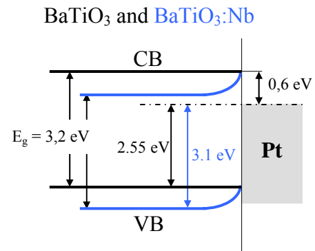
Figure 3.1.2.11: Experimentally determined energy band diagrams for BaTiO 3 /Pt and BaTiO 3 :Nb/Pt. The undoped film exhibits a flat band regime whereas a band bending appears at the interface with Nb doping. The barrier height in both cases is 0,6 eV.
