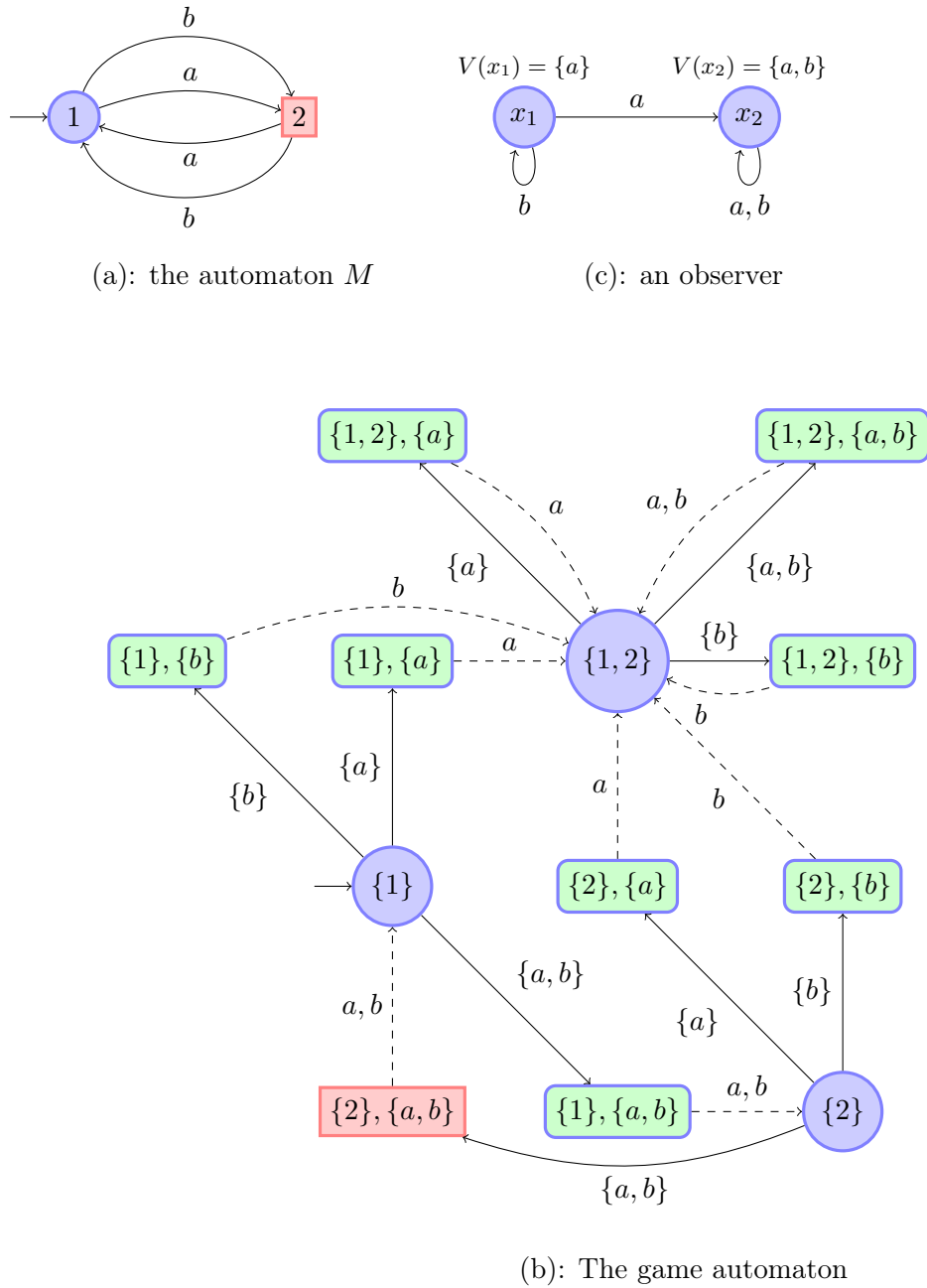
Figure 6.5: Example of a game automaton
