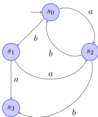
Figure 2.1: An example of LTS
