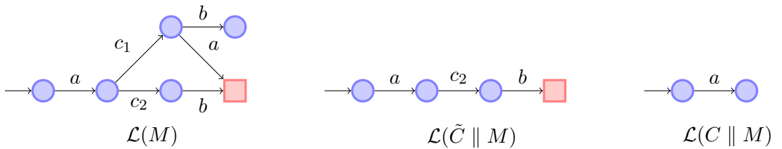
Figure 5.1: Removing disclosing words may introduce new vulnerabilities
