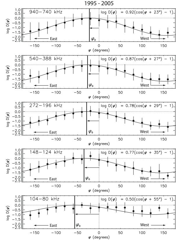
Fig. 4. The diagram in longitude \varphi relative to the source, with the fitted values of the amplitude a and shift \varphi_0 , is plotted as a continuous line as \log_{10}D(\varphi) vs. \varphi . The diagram data (see definition in the text) are averaged in 20^\circ bins of \varphi and plotted (black circles with scatter bars) vs. \varphi . As the frequency decreases, the shift \varphi_0 to east of the local magnetic field direction increases and the amplitude a of the cosine diagram decreases.
