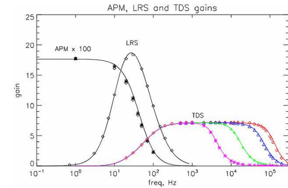
Fig. 15 The gain of the time domain parts of S/WAVES. Discrete points represent measurements. Lines represent theory. The negative APM gain (i.e. gain less than unity) is multiplied by 100 for visibility. Different TDS curves reflect selectable low pass filters
