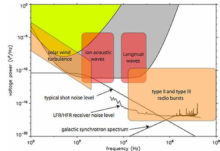
Fig. 4 (Color online) Required and known sensitivity as a function of frequency. Typical levels of solar wind electric field turbulence, ion acoustic, and Langmuir wave power are shown, as well as IP radio burst levels. The galactic nonthermal continuum level and the expected shot noise levels will determine the actual measurement background. The green area shows the expected sensitivity of the LRS burst measurement, while the grey area shows the expected TDS sensitivity. Measured LFR and HFR noise levels are also shown
