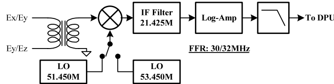
Fig. 12 FFR block diagram
