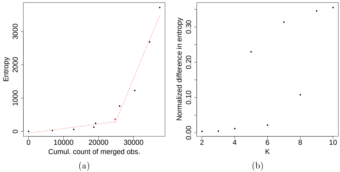
Figure 7.14: (a) Entropy values for the K-cluster Combined Solution for the GvHD Control Sample. The piecewise regression analysis suggests that K = 6 is the optimal number of clusters. (b) Differences between successive entropy values.
