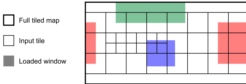
Figure 5.2: A dually tiled map. The map is a set of tiles of any size. We can load arbitrary windows of the map, even across the edges.
