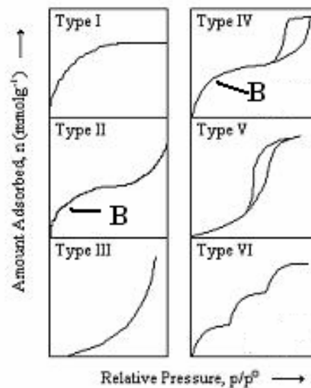
Figure II 14. Types d'isothermes de physisorption.
