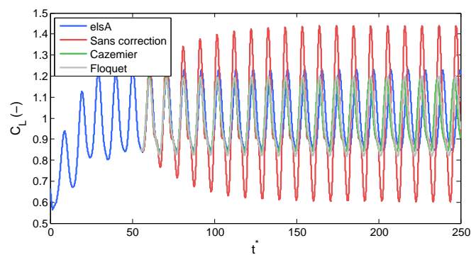
(b) Coefficient de portance
