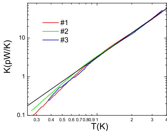
Fig. 2 (Color online) Thermal conductance measurements in log scale of three different nanowires with a section of 200 \times 100 \text{ nm}^2 and a length of 10 \mu\text{m} . Below 1.2 \text{ K} , the thermal conductance deviates from the higher temperature power law. The black line represents what is expected from the Casimir model (see (4))
